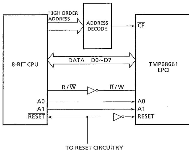
Figure 6.3 Interface Connections to 8-BIT CPU
