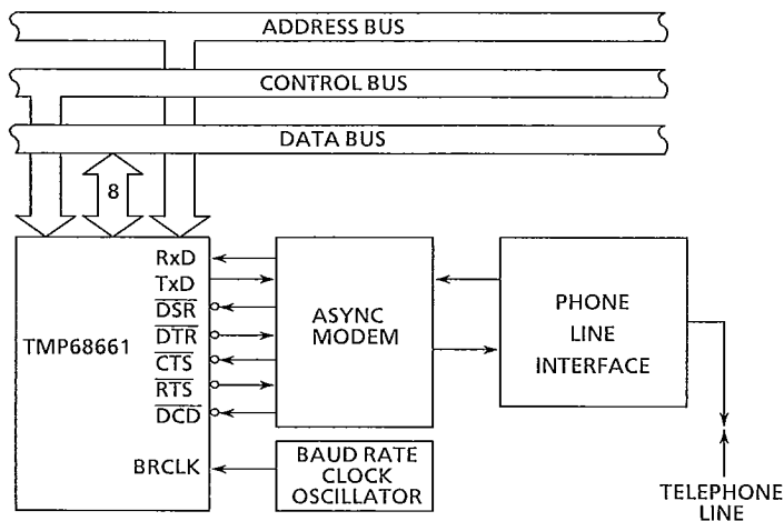
Figure 6.5 Asynchronous Interface to Telephone Lines
