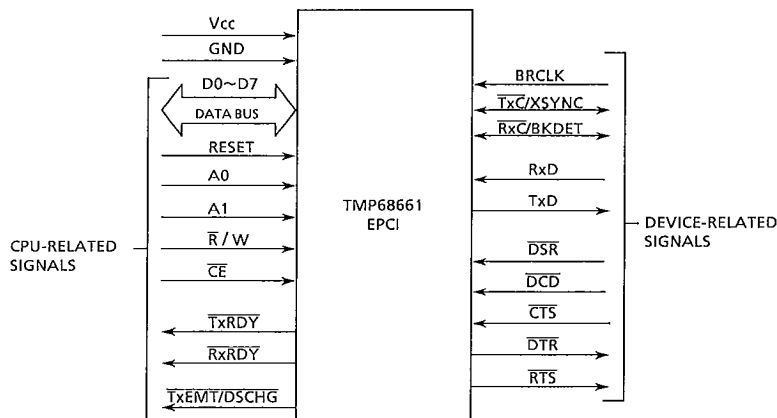
Figure 3.1 Input and Output Signals
