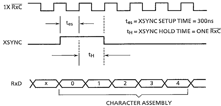
Figure 4.2 External Synchronization with XSYNC Timing Diagram
