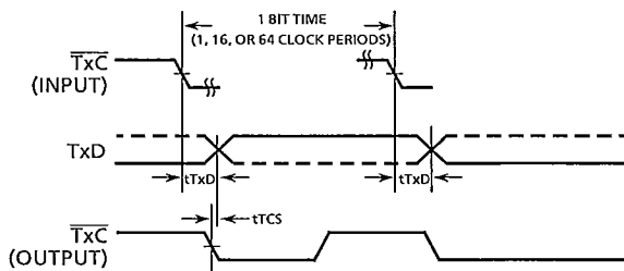
Figure 7.3 Transmit Timing Diagram
