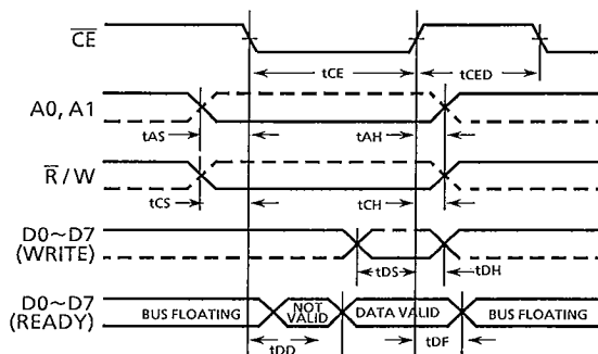
Figure 7.5 Read and Write Timing Diagram
