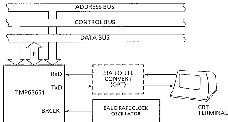
Figure 6.4 Asynchronous Interface to CRT Terminal
