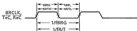
Figure 7.2 Clock Timing Diagram
