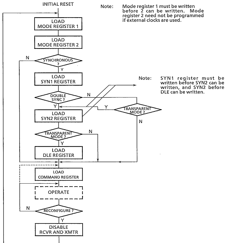
Figure 5.1 Initialization Flowchart
