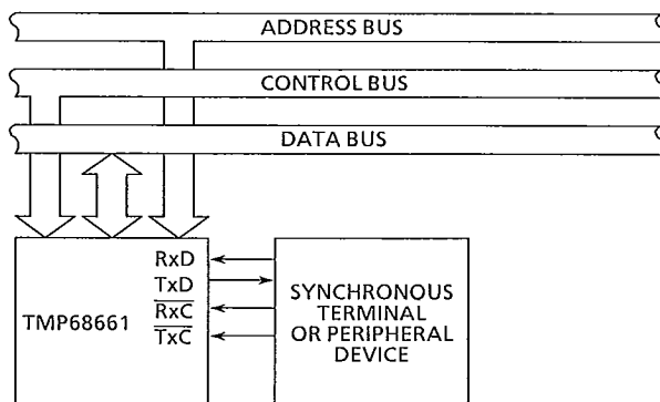
Figure 6.6 Synchronous Interface to Terminal or Peripheral Device
