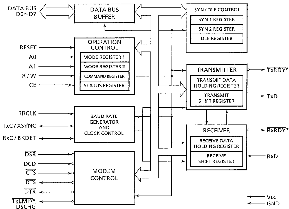
Figure 2.1 Block Diagram
