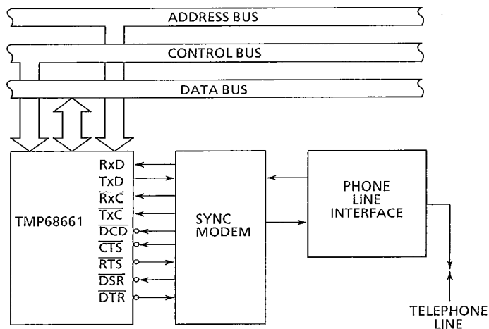
Figure 6.7 Synchronous Interface to Telephone Lines
