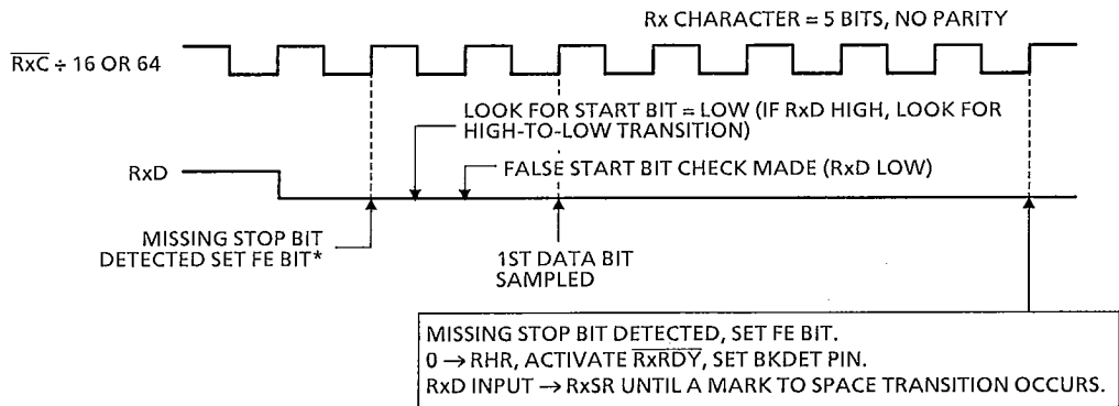
Figure 4.3 Break Detection Timing Diagram
