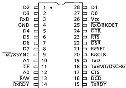
Figure 3.2 Pin Assignments
