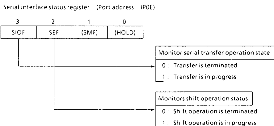
Figure 3-30. Serial Interface Status Register
