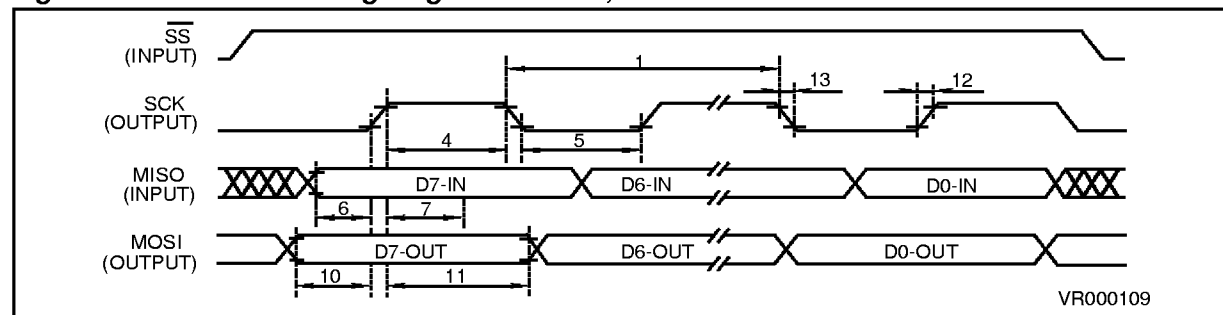
Figure 45. SPI Master Timing Diagram CPHA=0, CPOL=0
