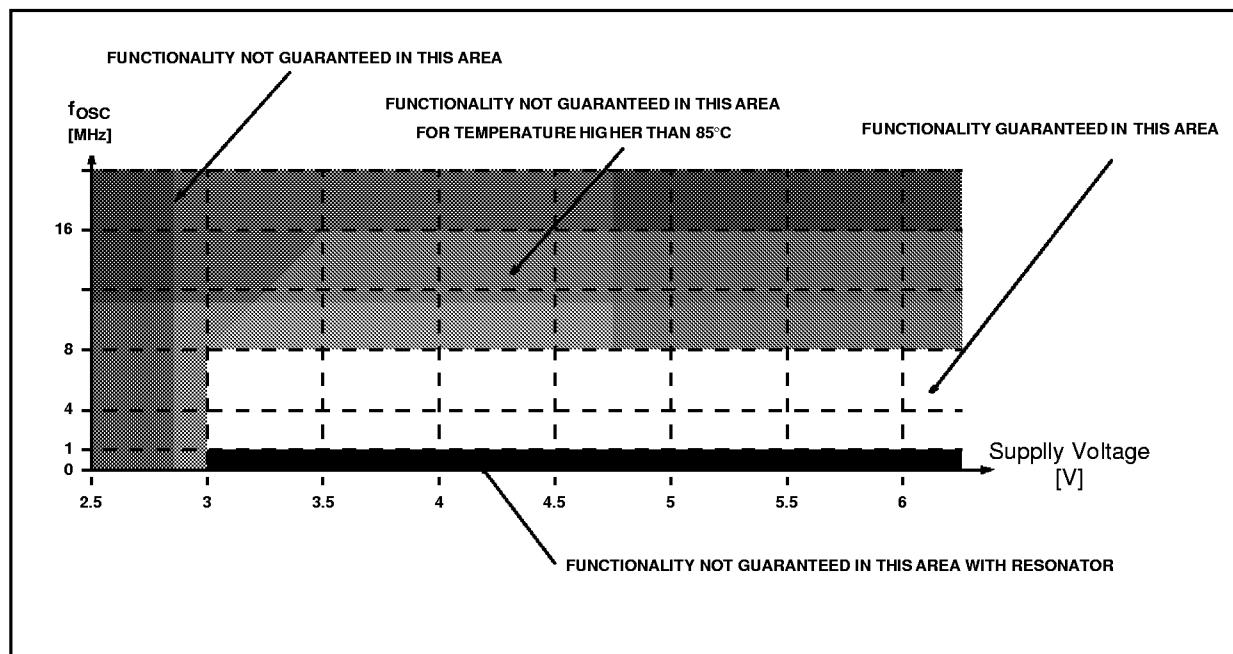
Figure 43. Maximum Operating Frequency ( f_{OSC} ) Versus Supply Voltage ( V_{DD} )
