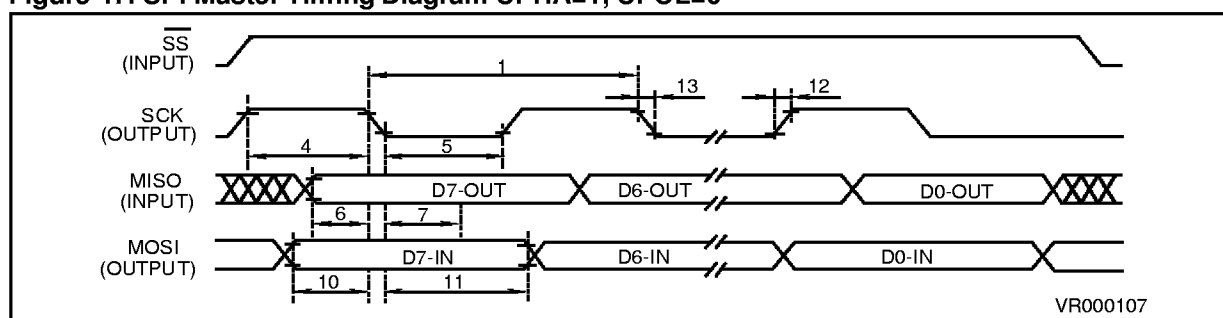
Figure 47. SPI Master Timing Diagram CPHA=1, CPOL=0
