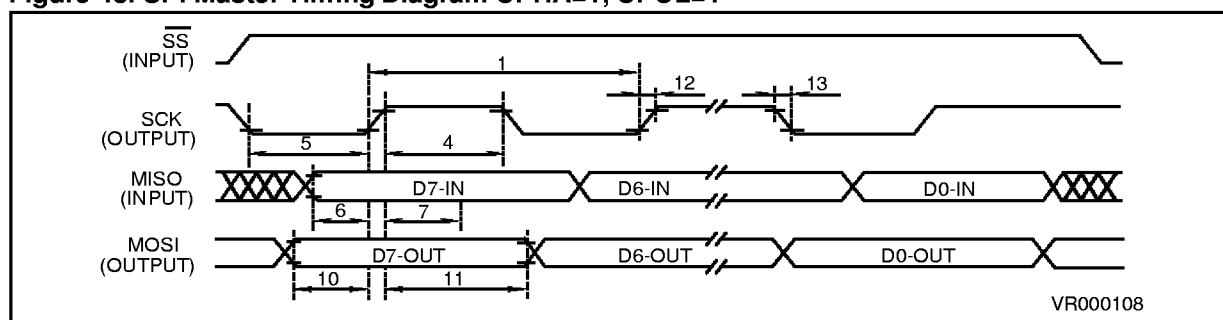
Figure 48. SPI Master Timing Diagram CPHA=1, CPOL=1
