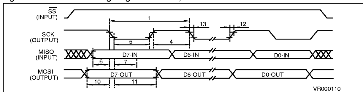
Figure 46. SPI Master Timing Diagram CPHA=0, CPOL=1
