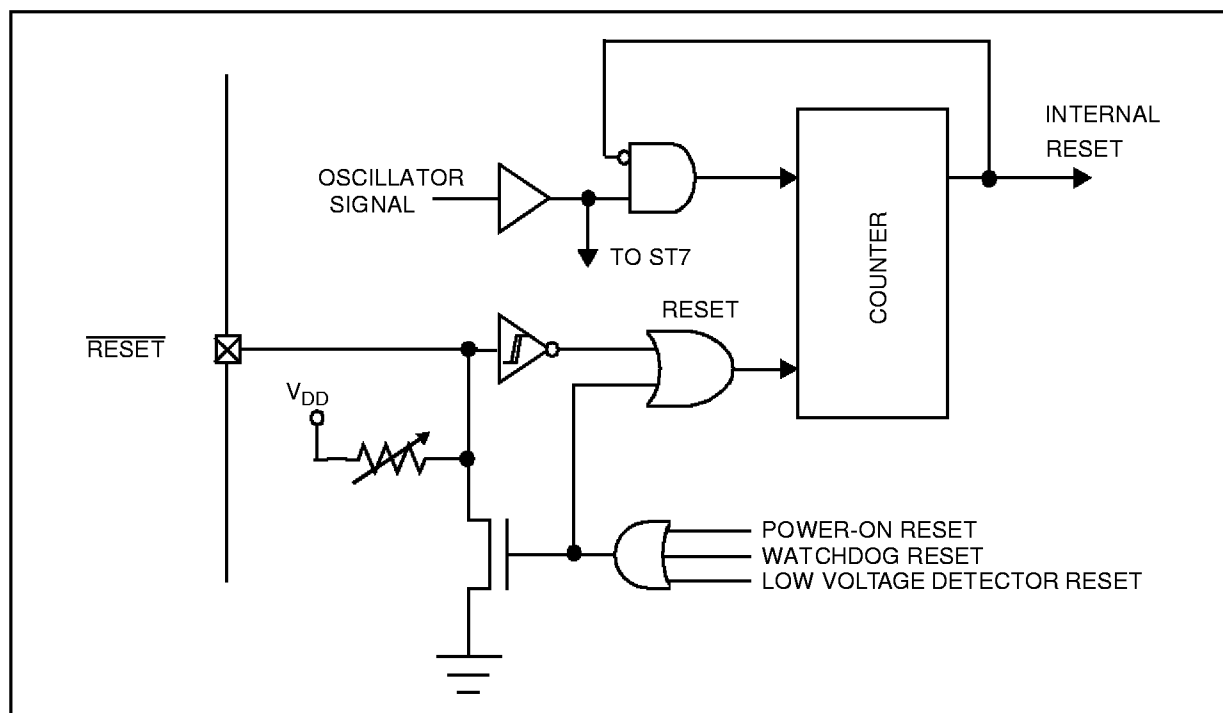
Figure 12. Reset Block Diagram
