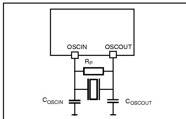
Figure 10. Crystal/Ceramic Resonator
