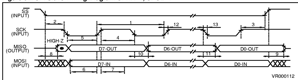
Figure 52. SPI Slave Timing Diagram CPHA=1, CPOL=1
