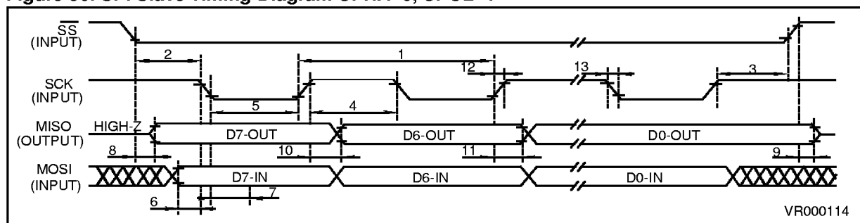
Figure 51. SPI Slave Timing Diagram CPHA=1, CPOL=0
