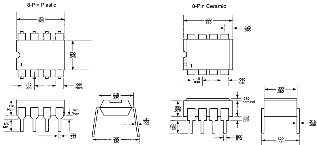
Figure 9. Package Dimensions
