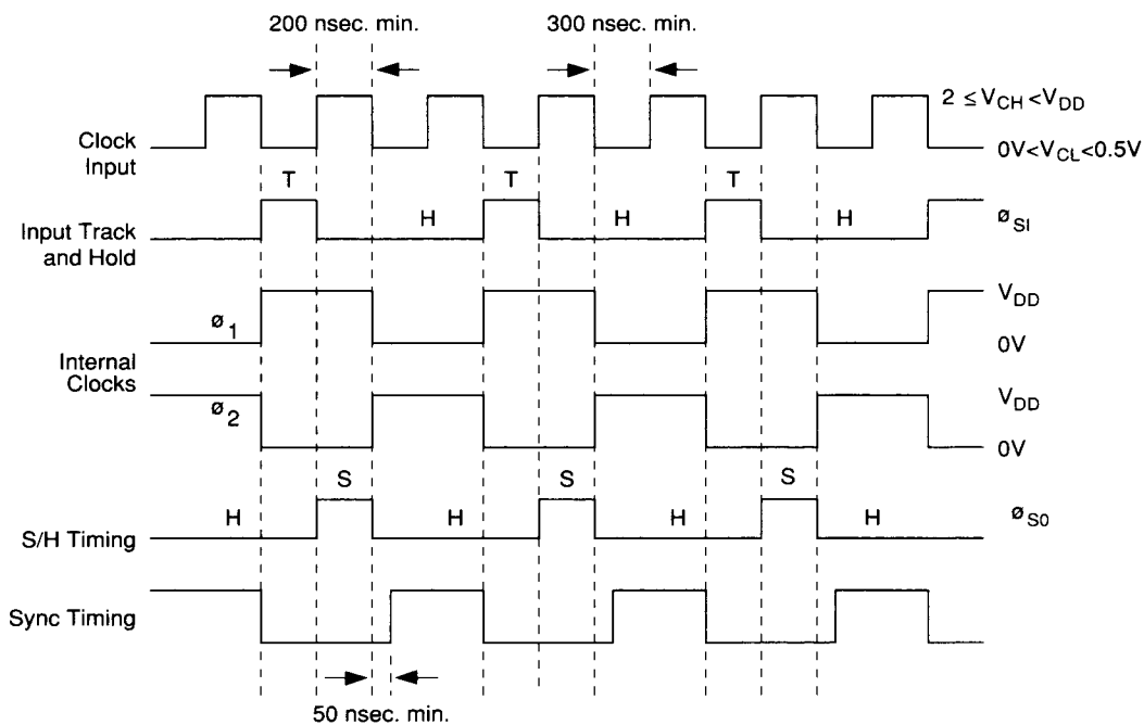
Figure 4. Timing Relations
