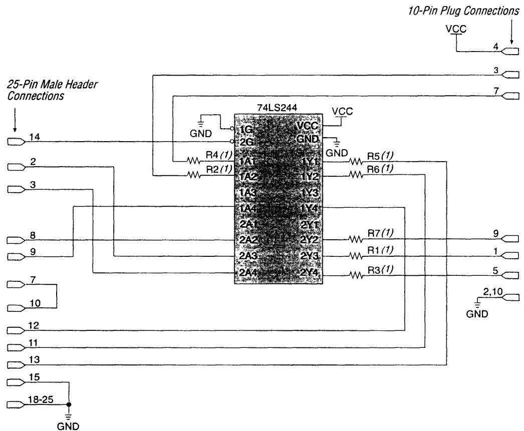
Figure 2. ByteBlaster Schematic
