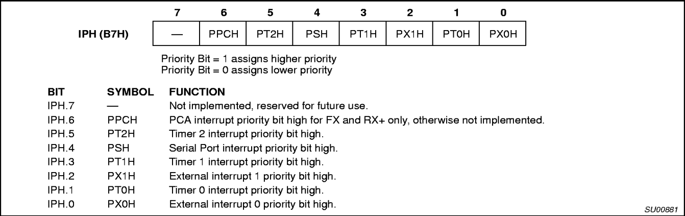
Figure 12. IPH Registers
