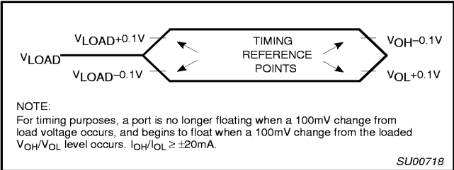
Figure 20. Float Waveform
