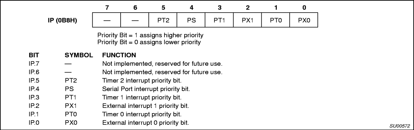
Figure 11. IP Registers
