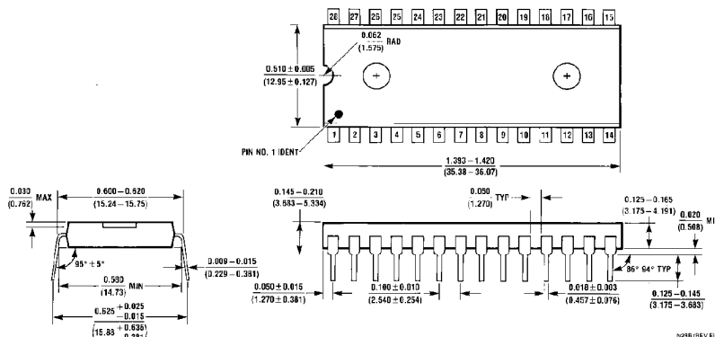
Dual-In-Line Package (N) Order Number NMC27C64N NS Package Number N28B
