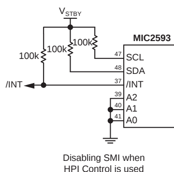
Figure 6. Input Pin Configuration for Disabling HPI/SMI Control
