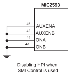
Figure 6. Input Pin Configuration for Disabling HPI/SMI Control
