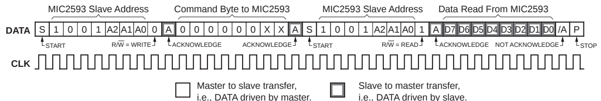
Figure 10. READ_BYTE Protocol
