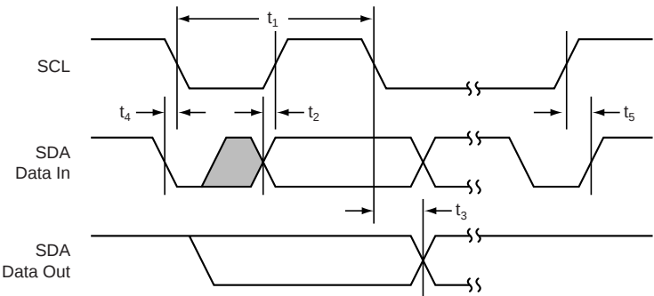
Figure 1. SMBus Timing
