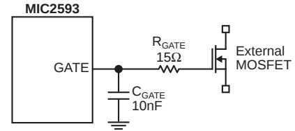
Figure 15. C_{GATE} and R_{GATE} Connection
