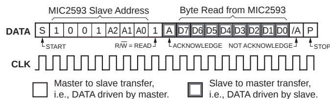
Figure 11. RECEIVE_BYTE Protocol
