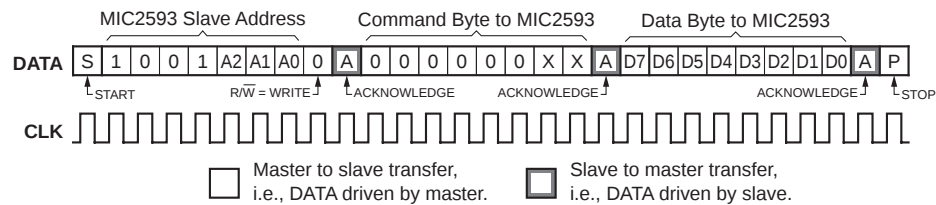
Figure 9. WRITE_BYTE Protocol
