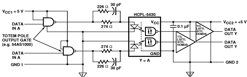
Figure 15. Recommended HCPL-5430 and HCPL-6430 Interface Circuit.
