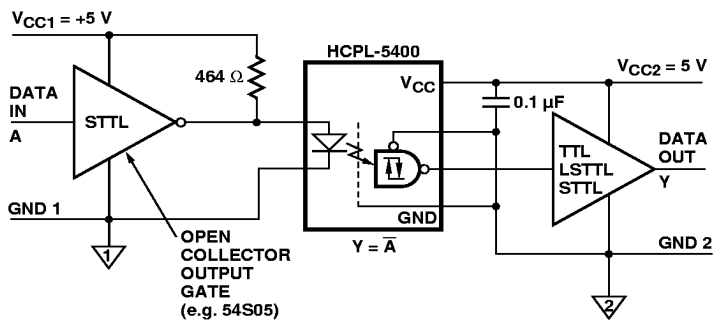
Figure 14. Alternative HCPL-5400 Interface Circuit.
