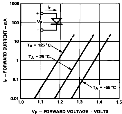
Figure 4. Typical Diode Input Forward Current Characteristic.
