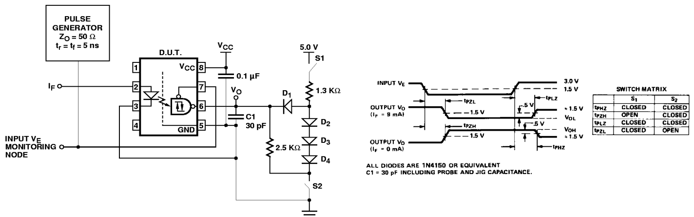
Figure 8. Test Circuit for t_{PHZ} , t_{PZH} , t_{PLZ} , and t_{PZL} . (Single Channel Product Only).
