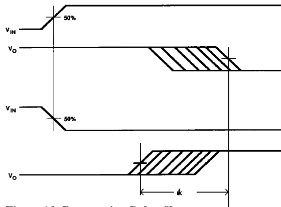
Figure 10. Propagation Delay Skew, t_{PSK} , Waveform.
