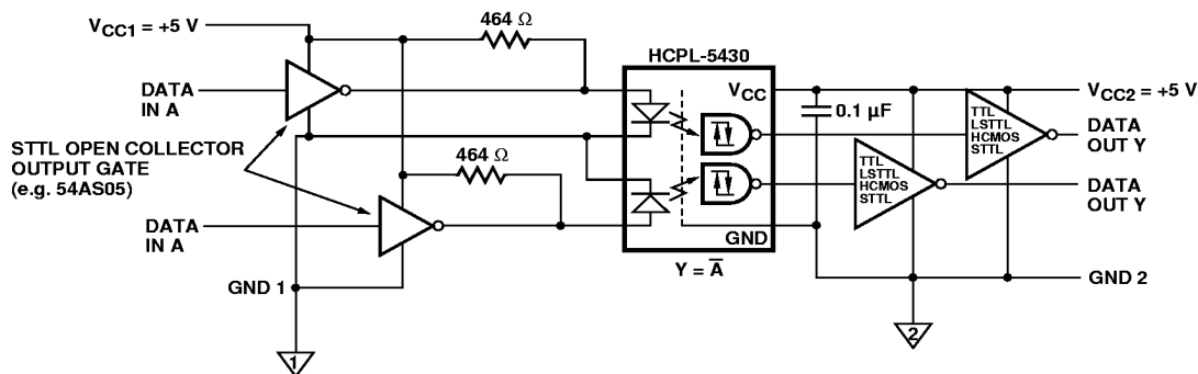
Figure 16. Alternative HCPL-5430 and HCPL-6430 Interface Circuit.
