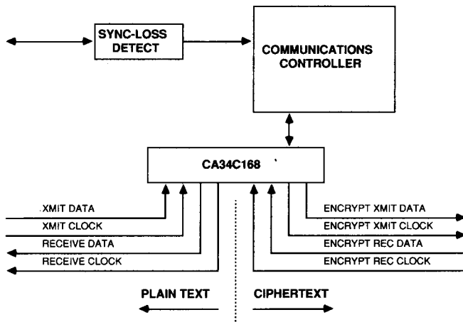
Figure 28 : STREAM CIPHER
