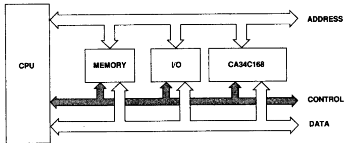
Figure 24 : MICROPROCESSOR INTERFACE for BLOCK TRANSFERS
