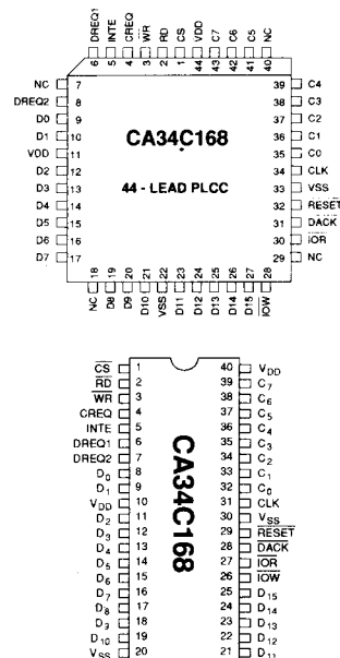
Figure 2 : PLCC and DIP PIN CONFIGURATIONS
