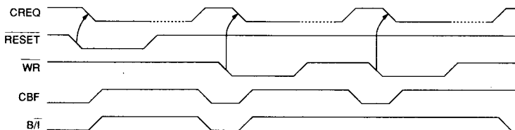
Figure 16 : WRITING DEP INSTRUCTIONS
