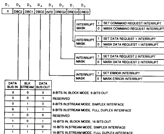
Figure 10: MODE REGISTER ASSIGNMENTS
