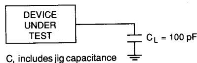
Figure 8: AC TESTING LOAD CIRCUIT
