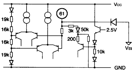
MUTE CTRL
