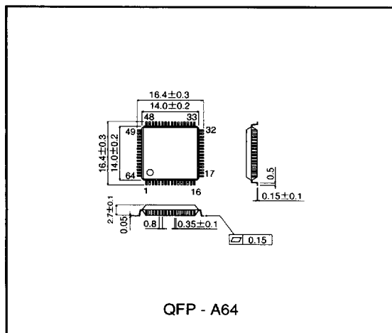
●External dimensions (Units: mm)
