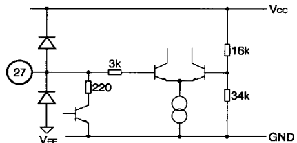
FNORM DLY
