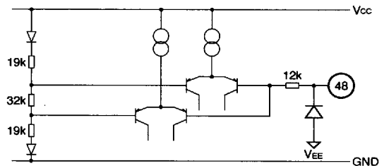
FNORM DLY
