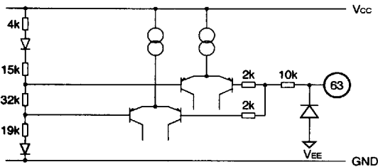
MUTE CTRL
