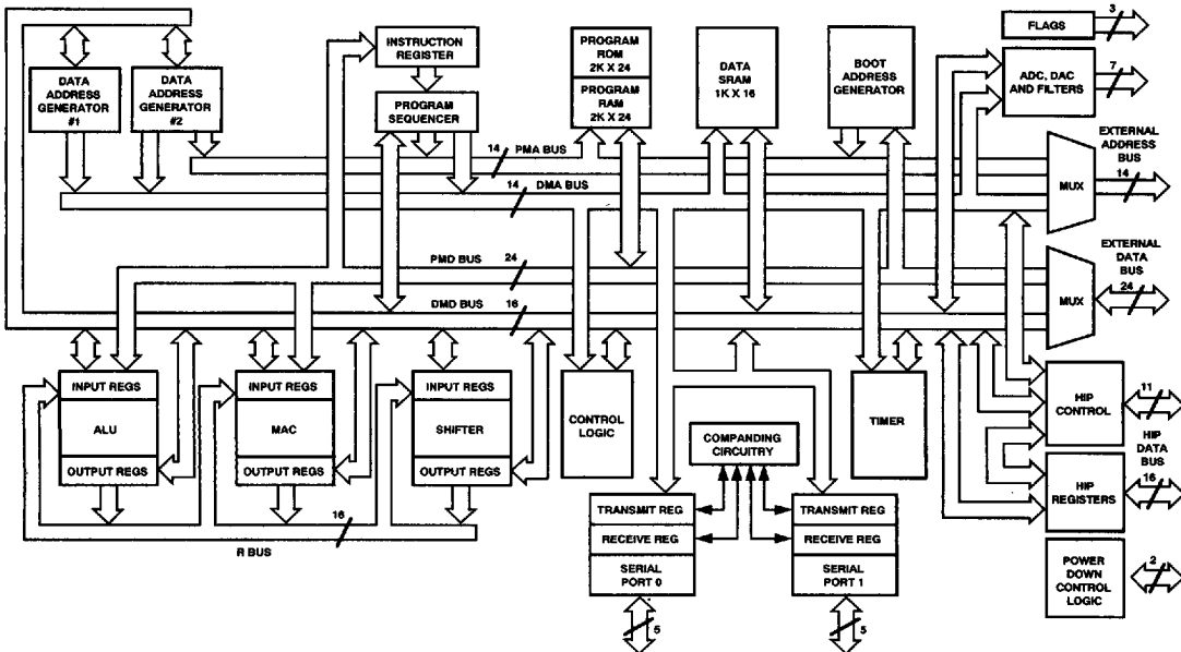
Figure 1. ADSP-21msp5xA Block Diagram
