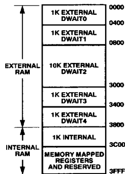
Figure 7. ADSP-21msp5xA Data Memory Map
