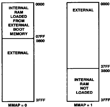
Figure 5. ADSP-21msp50A/55A Program Memory Maps
