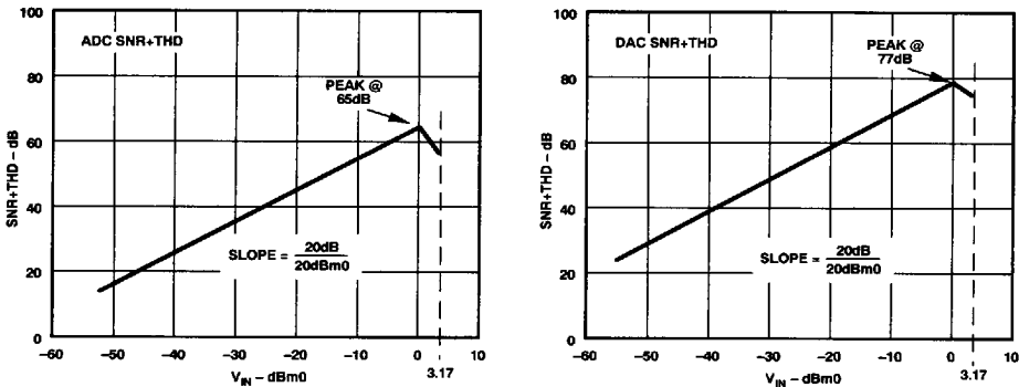
Figure 14. SNR + THD vs. V IN
