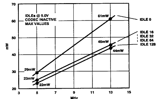
Figure 25. Power vs. Frequency
