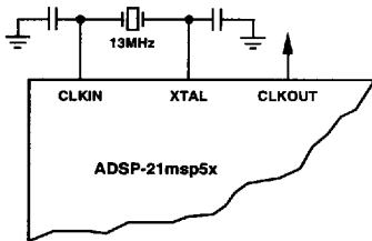
Figure 4. External Crystal Connections
