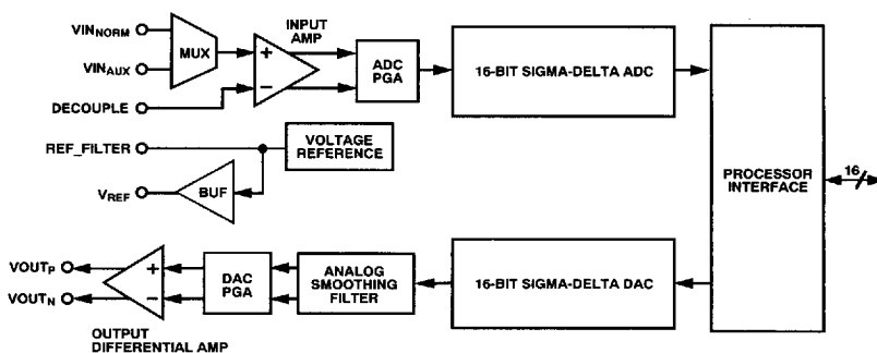
Figure 8. Analog Interface Block Diagram
