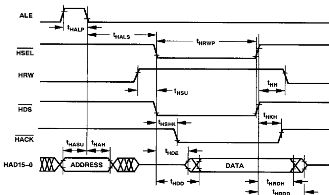
Figure 24. Host Interface Port (HMD1 = 1, HMD0 = 1)
