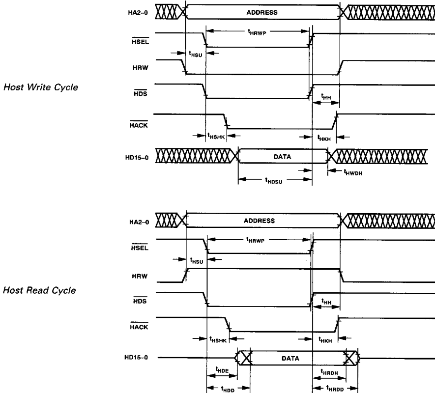
Figure 22. Host Interface Port (HMD1 = 0, HMD0 = 1)
