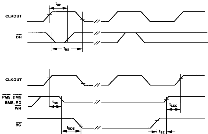
Figure 17. Bus Request – Bus Grant
