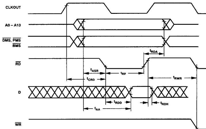
Figure 18. Memory Read
