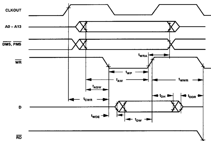
Figure 19. Memory Write
