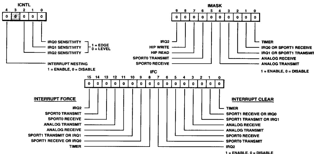
Figure 2. Interrupt Registers
