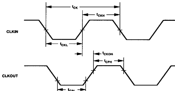
Figure 15. Clock Signals
