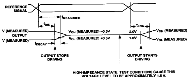
Figure 31. Output Enable/Disable
