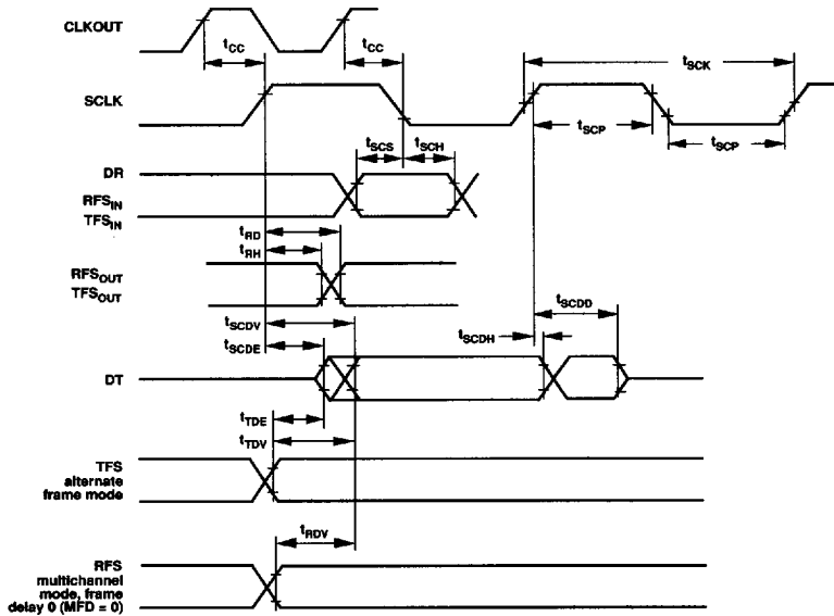
Figure 20. Serial Ports
