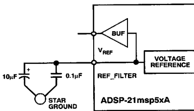
Figure 13. Voltage Reference Filter Capacitor
