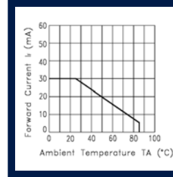
DERATING CURVE
