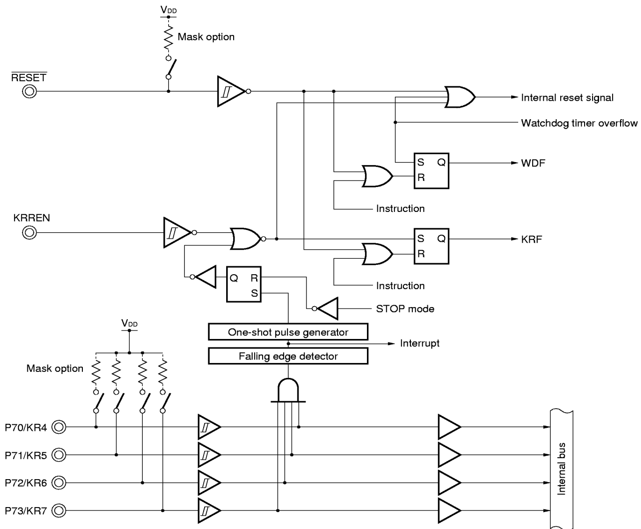
Figure 9-1. Configuration of Reset Function
