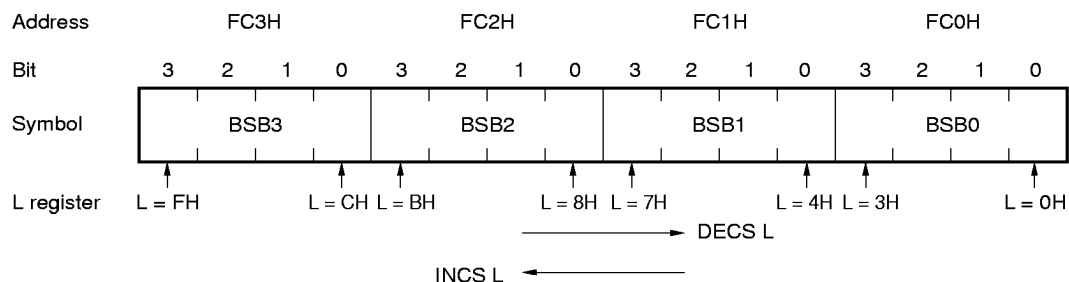
Figure 6-6. Bit Sequential Buffer Format
