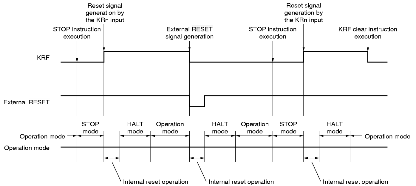
Figure 9-4. KRF Operation in Generating Each Signal
