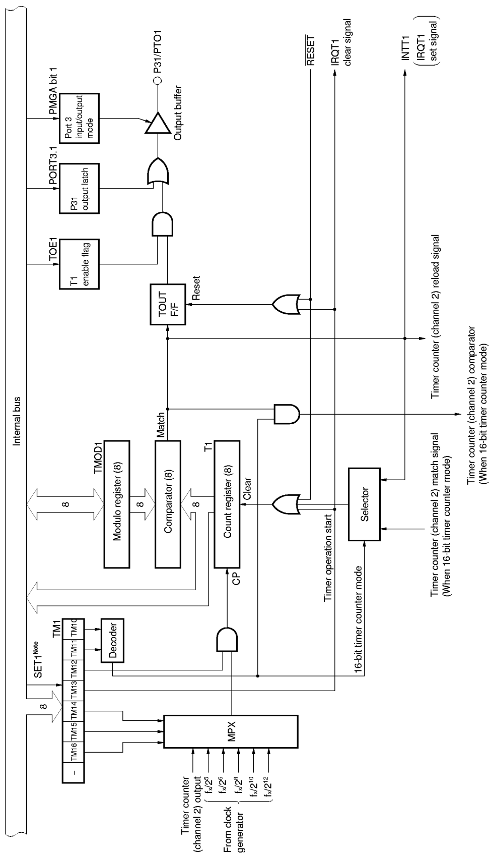
Figure 6-4. Timer Counter (Channel 1) Block Diagram
