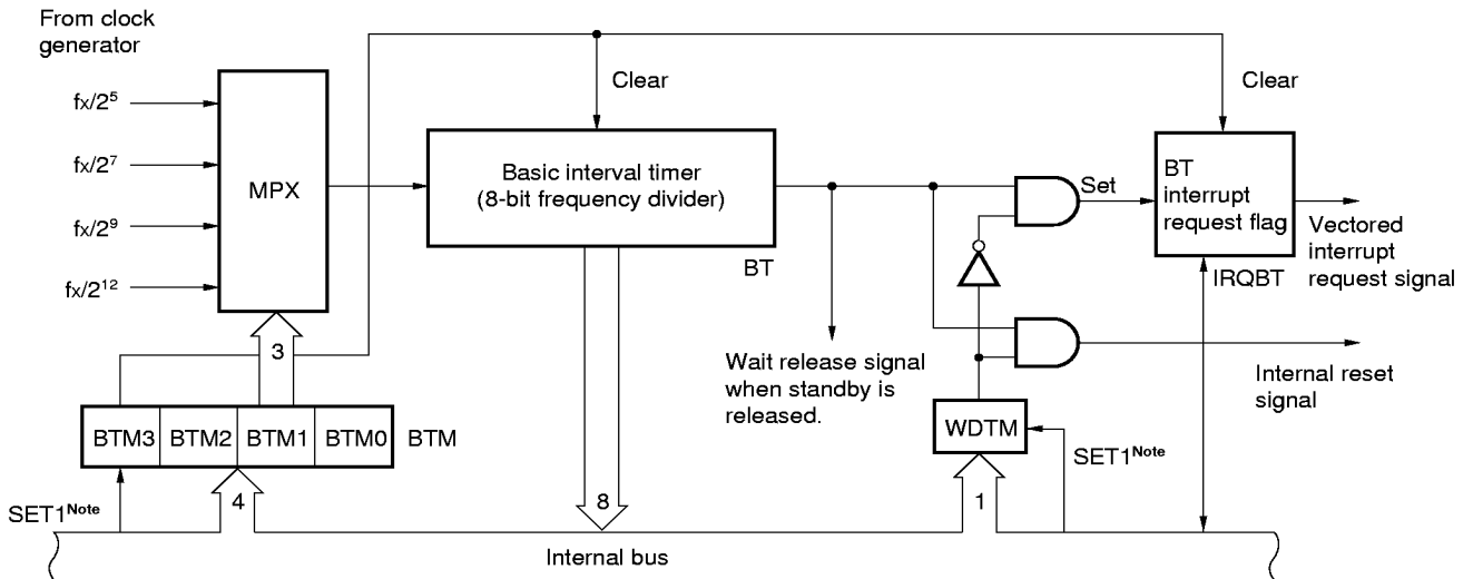
Figure 6-2. Basic Interval Timer/Watchdog Timer Block Diagram
