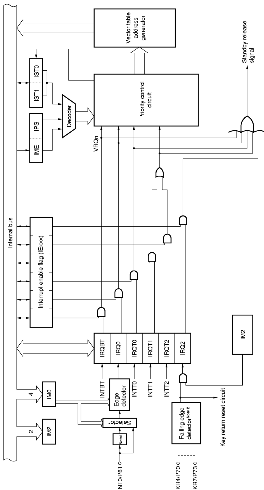
Figure 7-1. Interrupt Control Circuit Block Diagram
