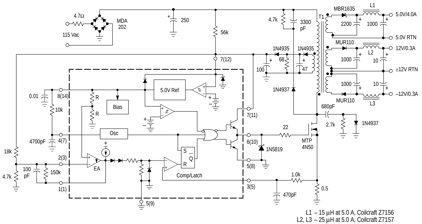
Figure 33. 27 W Off-Line Flyback Regulator
