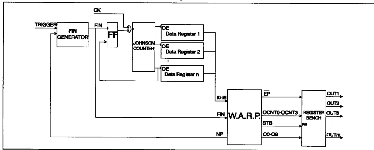
Figure 10. Input/Output Connection Block Diagram
