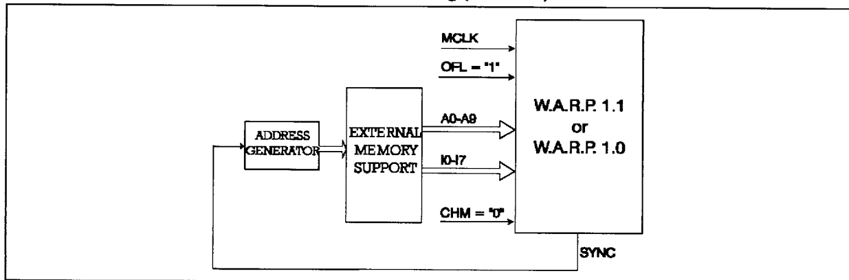
Figure 8. Block Diagram for W.A.R.P. downloading (CHM "0")
