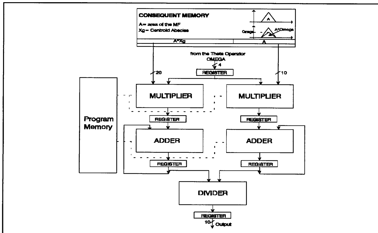
Figure 7. Defuzzifier Structure
