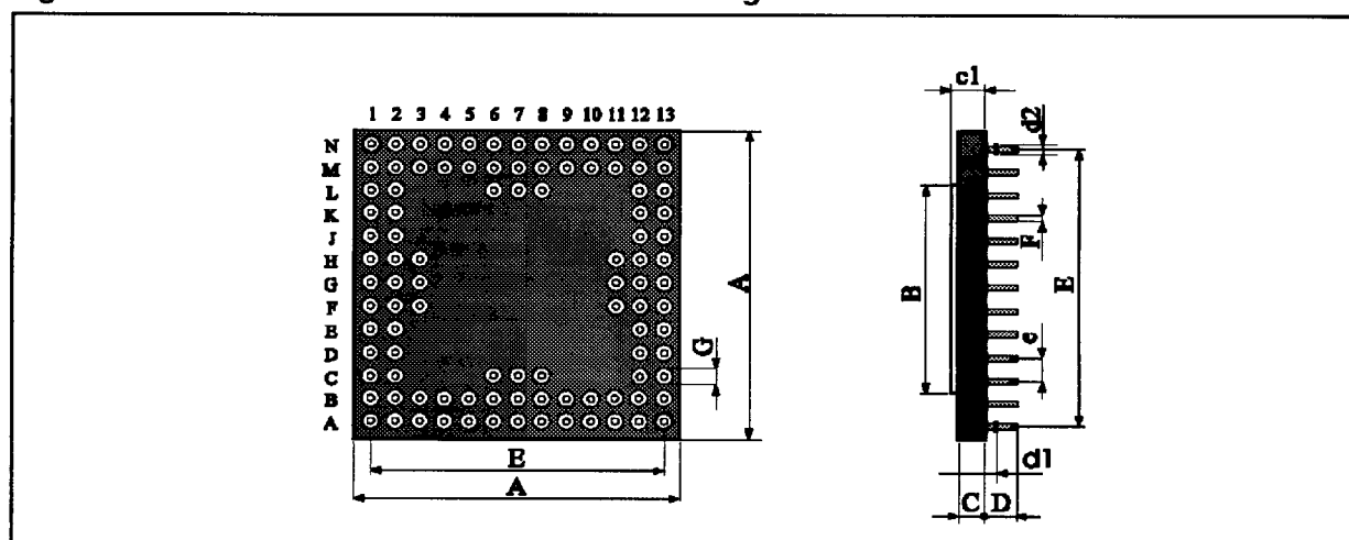
Figure 14. W.A.R.P. 100 Pin CPGA100 Ceramic Package
