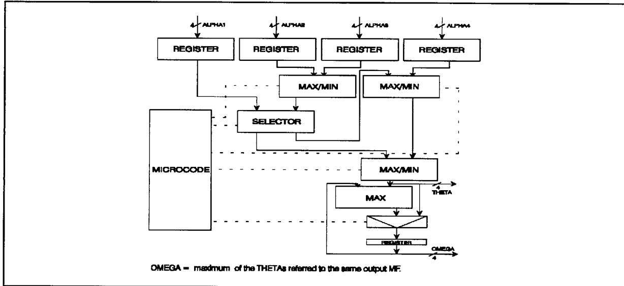
Figure 6. Inference Unit Structure
