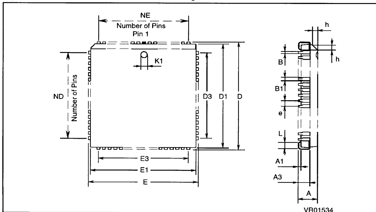
Figure 13. W.A.R.P. 84 Pin PLCC84 Plastic Package
