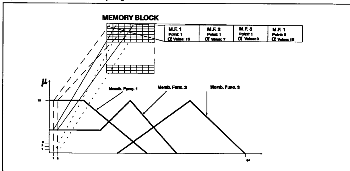
Figure 5. Antecedent Memory Organization
