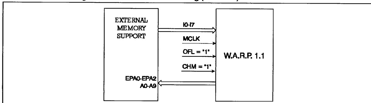
Figure 9. Block Diagram for W.A.R.P. downloading (CHM "1")
