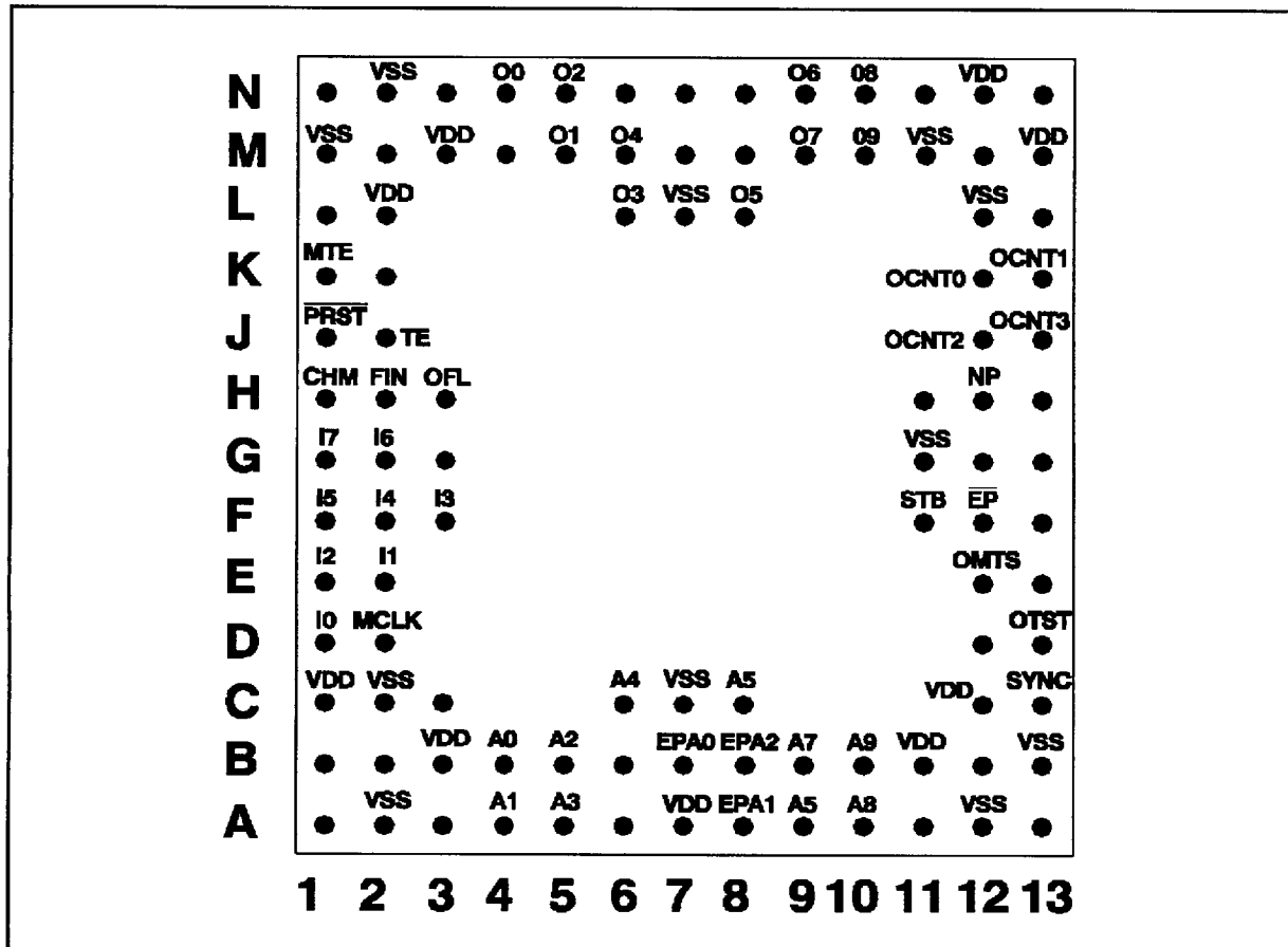
Figure 2. CPGA100 Pin Configuration
