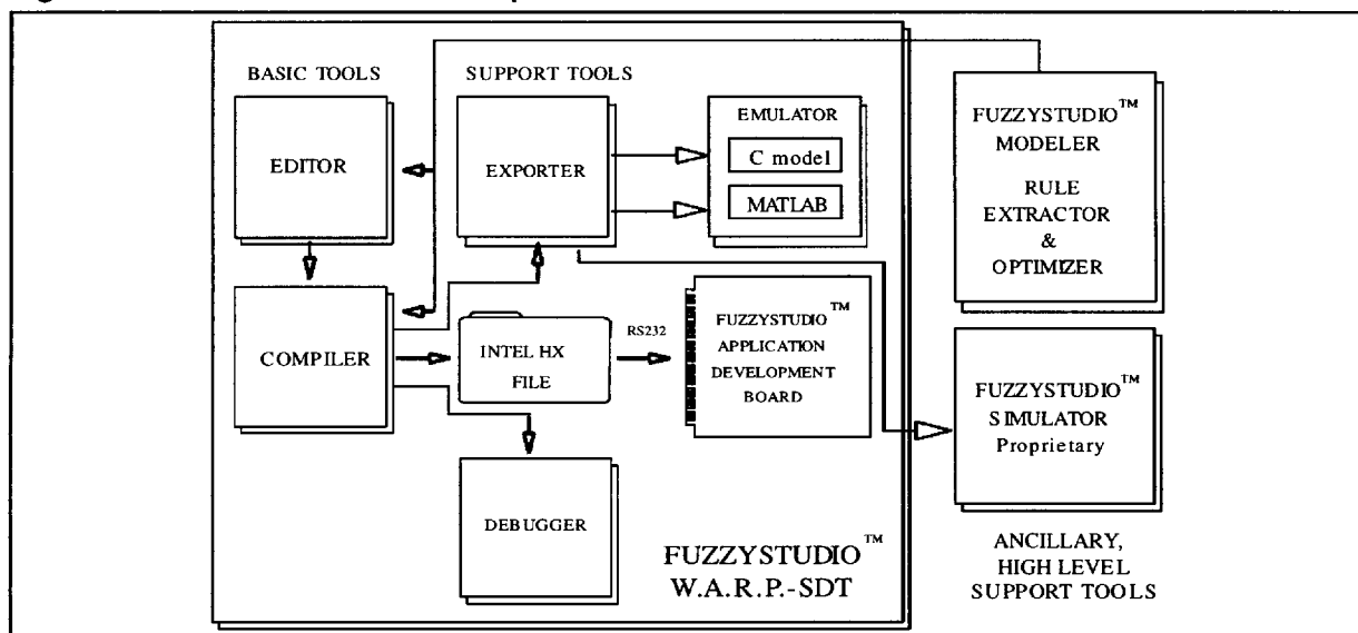
Figure 11. W.A.R.P. Software Development Tools
