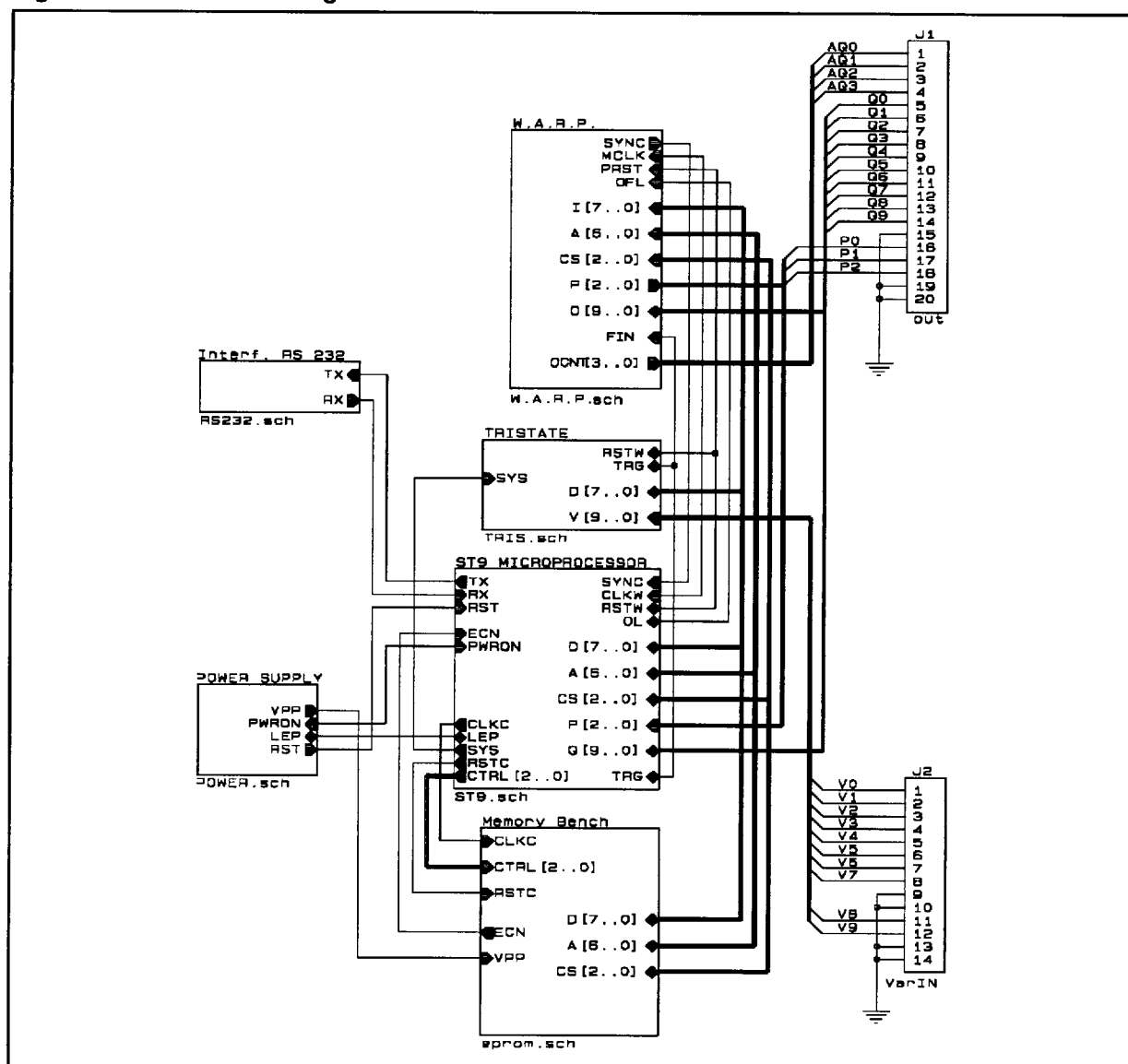
Figure 12. Board Block Diagram
