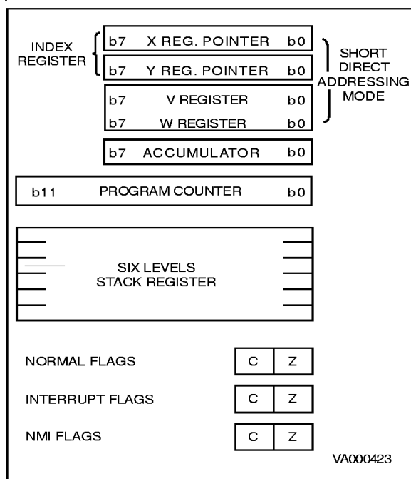
Figure 7. ST6 CPU Programming Mode
