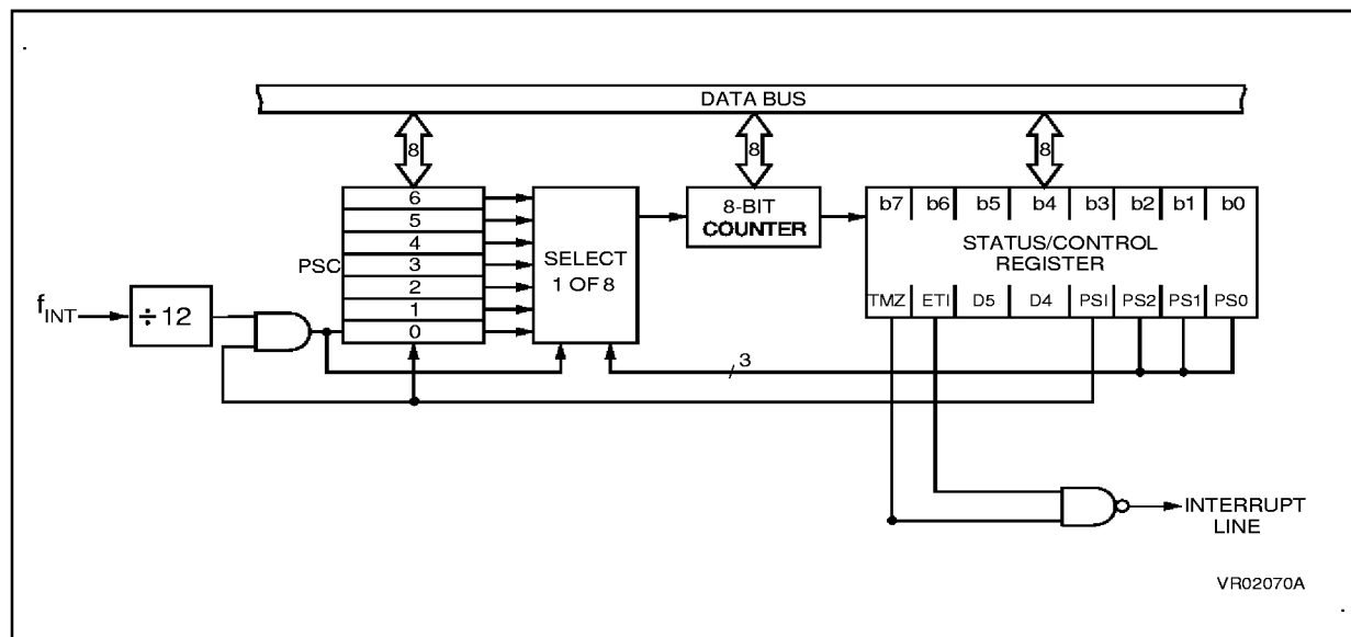
Figure 23. TIMER 2 Block Diagram
