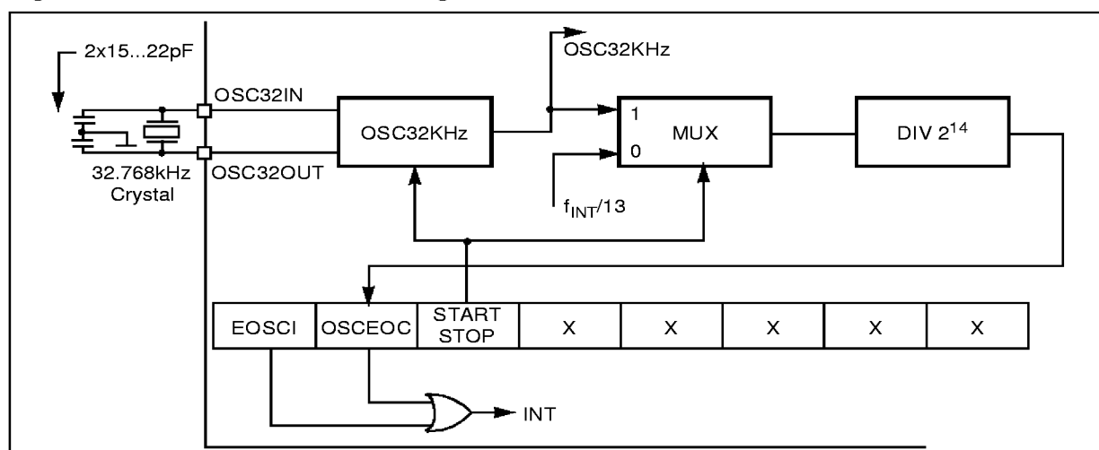
Figure 10. 32kHz Oscillator Block Diagram
