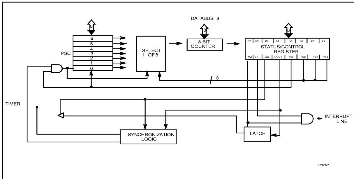
Figure 23. TIMER 2 Block Diagram
