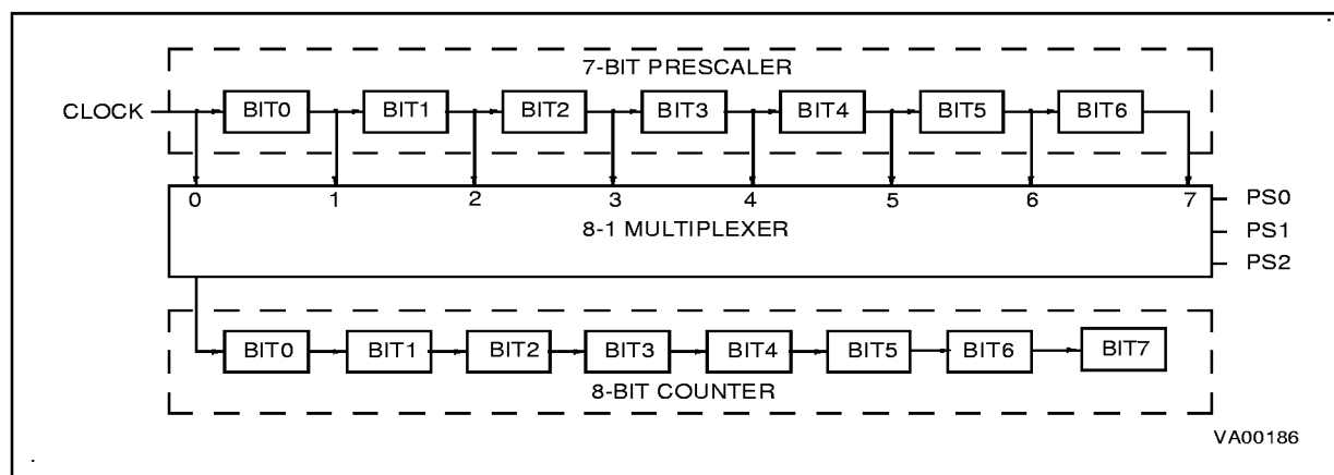
Figure 21. Timer Working Principle
