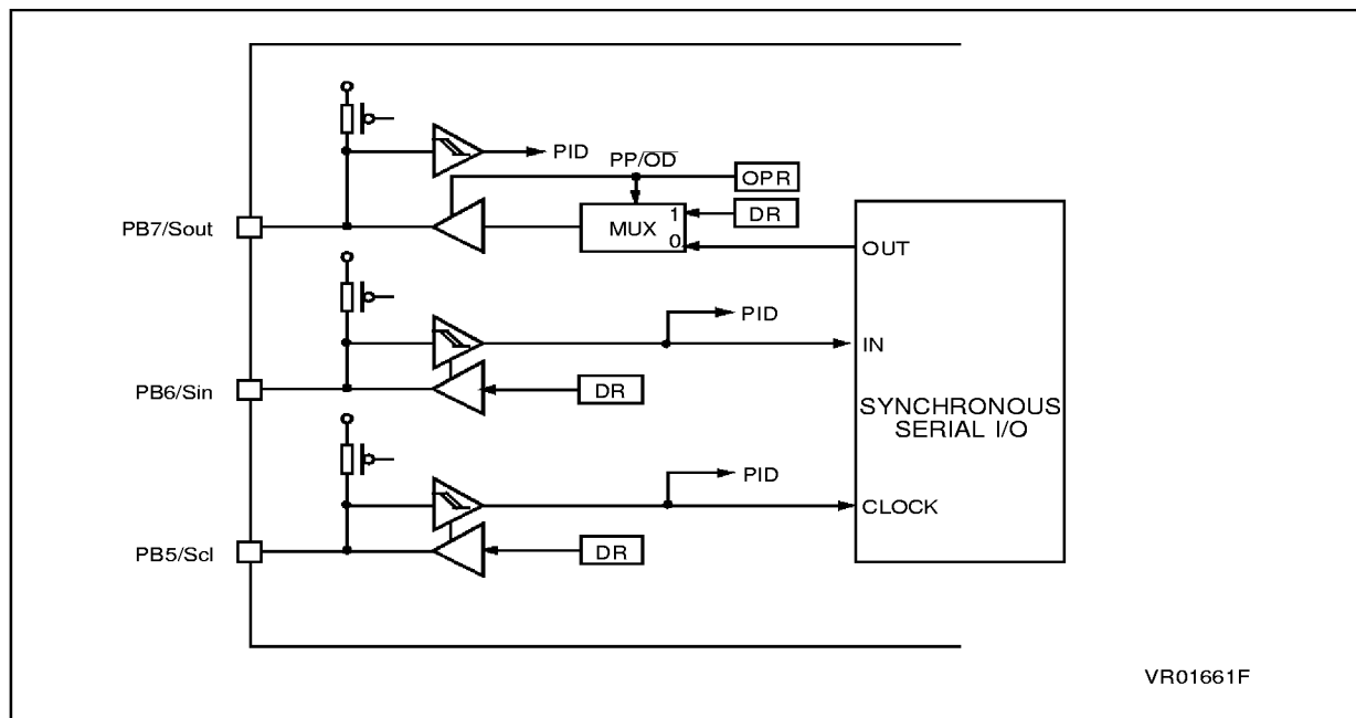
Figure 20. Peripheral Interface Configuration of SPI
