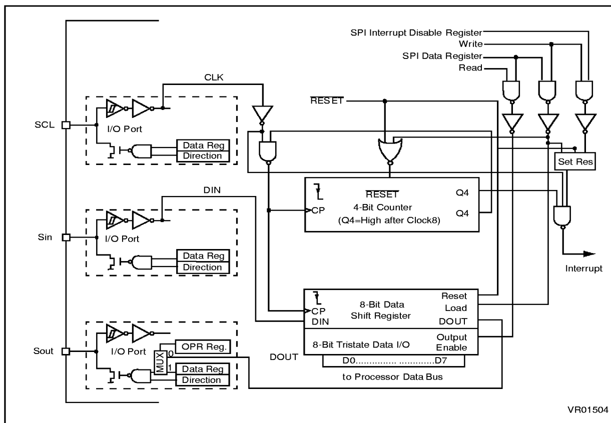
Figure 25. SPI Block Diagram
