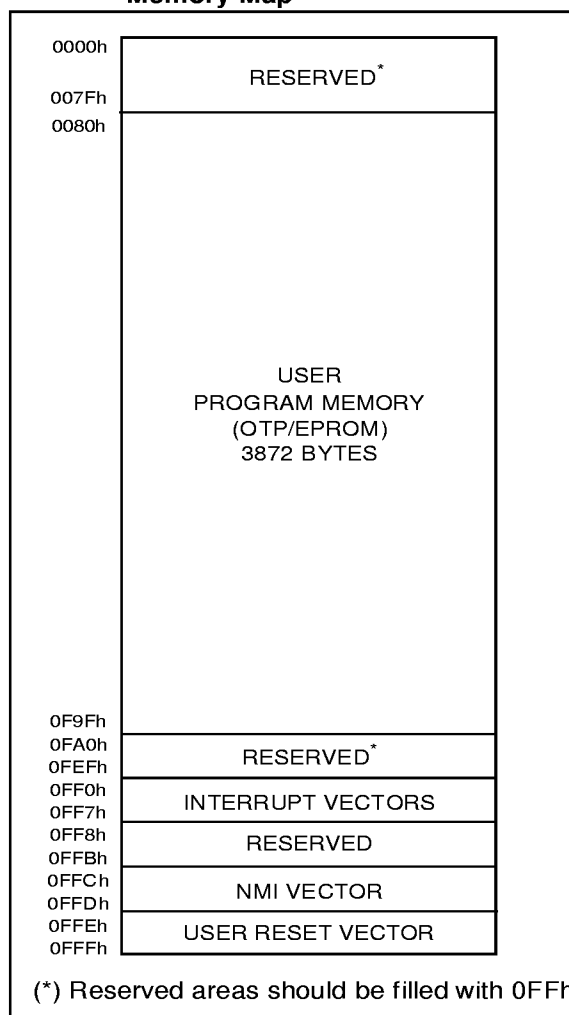
Figure 4. ST62E45B/T45B Program Memory Map
