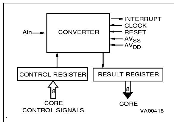
Figure 24. ADC Block Diagram
