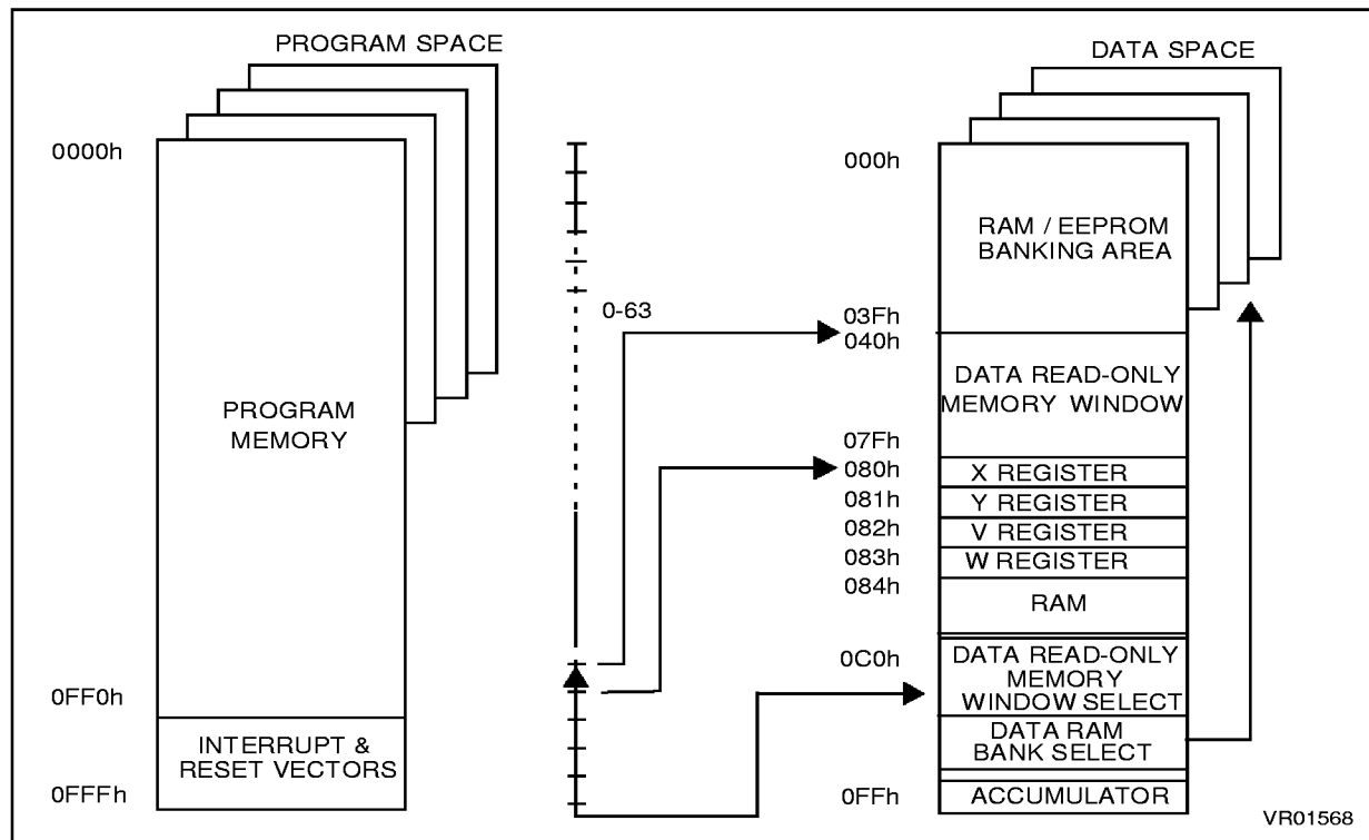
Figure 3. Memory Addressing Diagram
