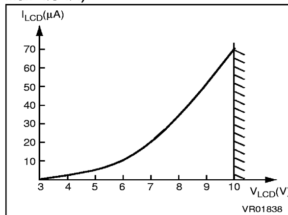
Figure 28. Typical Current consumption on VLCD Pin (25°C, no load, f_{LCD}=512Hz , mux=1/3-1/4)
