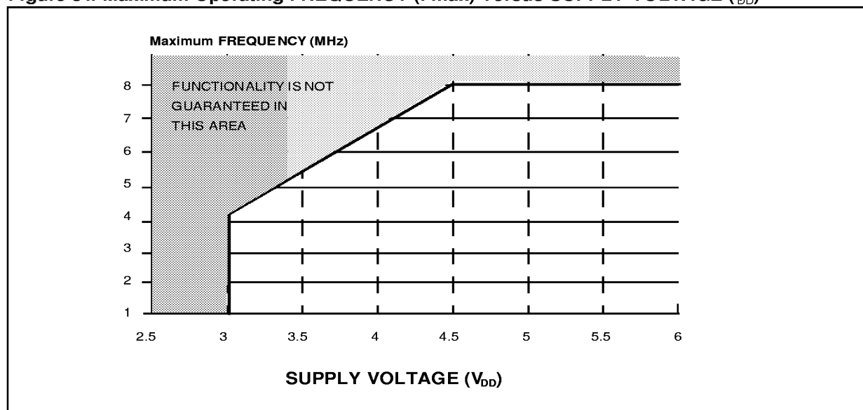
Figure 31. Maximum Operating FREQUENCY (Fmax) Versus SUPPLY VOLTAGE ( V_{DD} )
