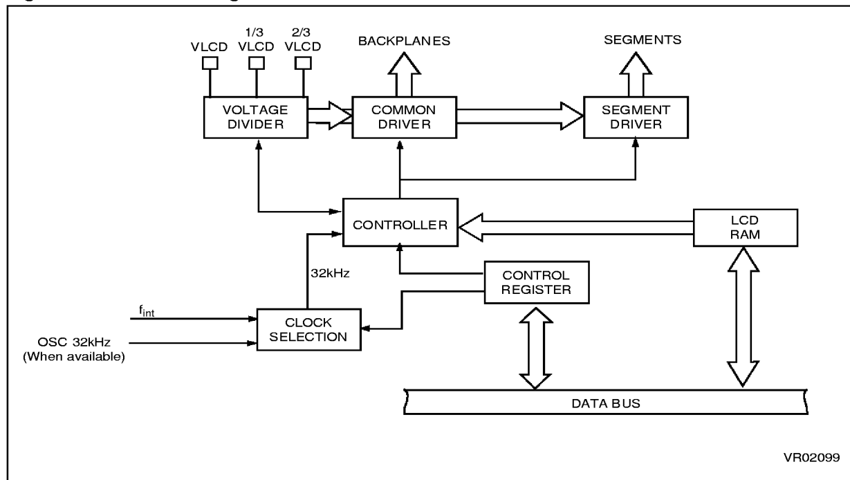
Figure 26. LCD Block Diagram
