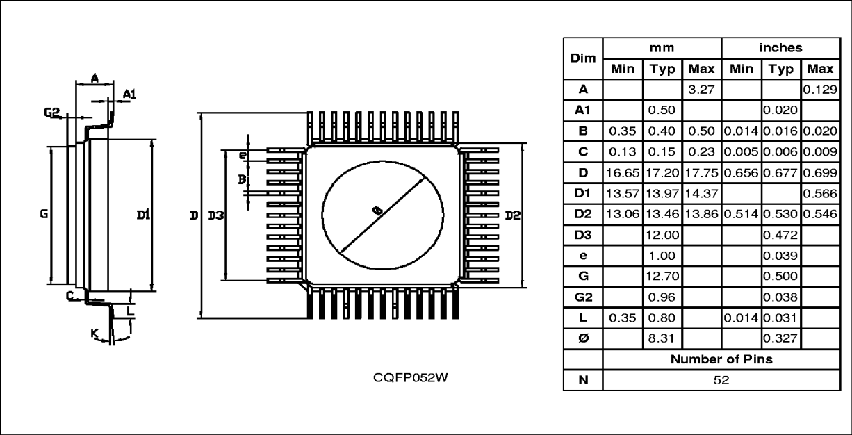
Figure 33. 52-Pin Ceramic Quad Flat Package with Window
