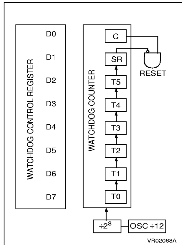
Figure 14. Watchdog Counter Control
