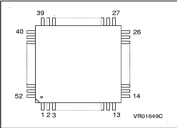
Figure 2. 52 Pin QFP Package
