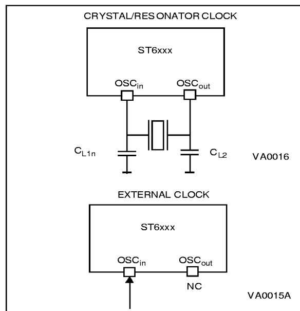
Figure 8. Oscillator Configurations
