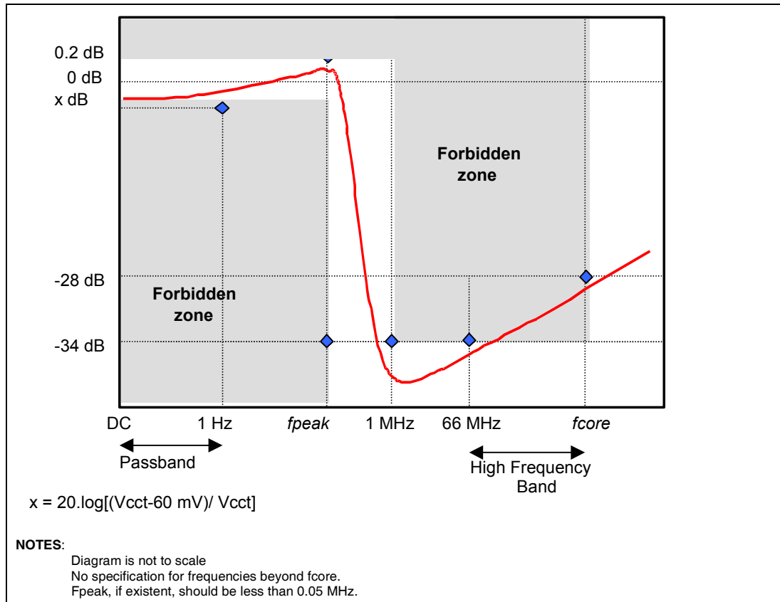
Figure 32. PLL Filter Specifications
