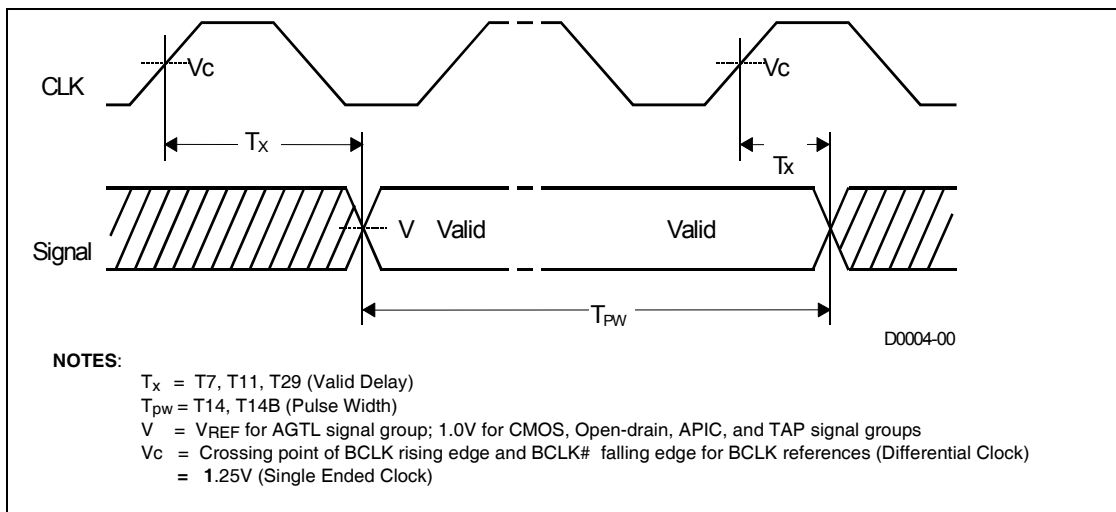
Figure 12. Valid Delay Timings
