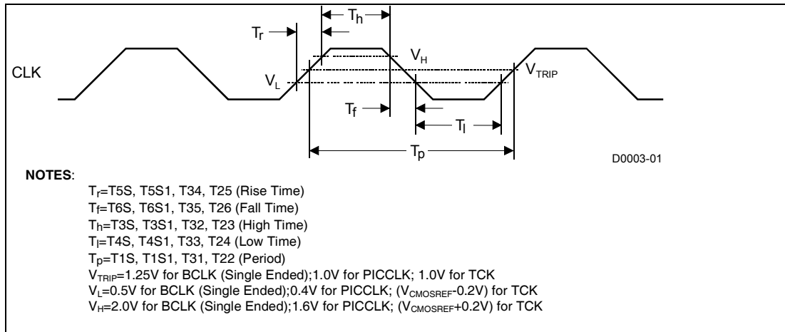
Figure 9. BCLK (Single Ended)/PICCLK/TCK Generic Clock Timing Waveform
