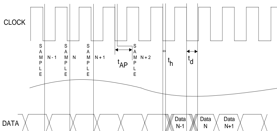
Figure 4. Timing diagram
