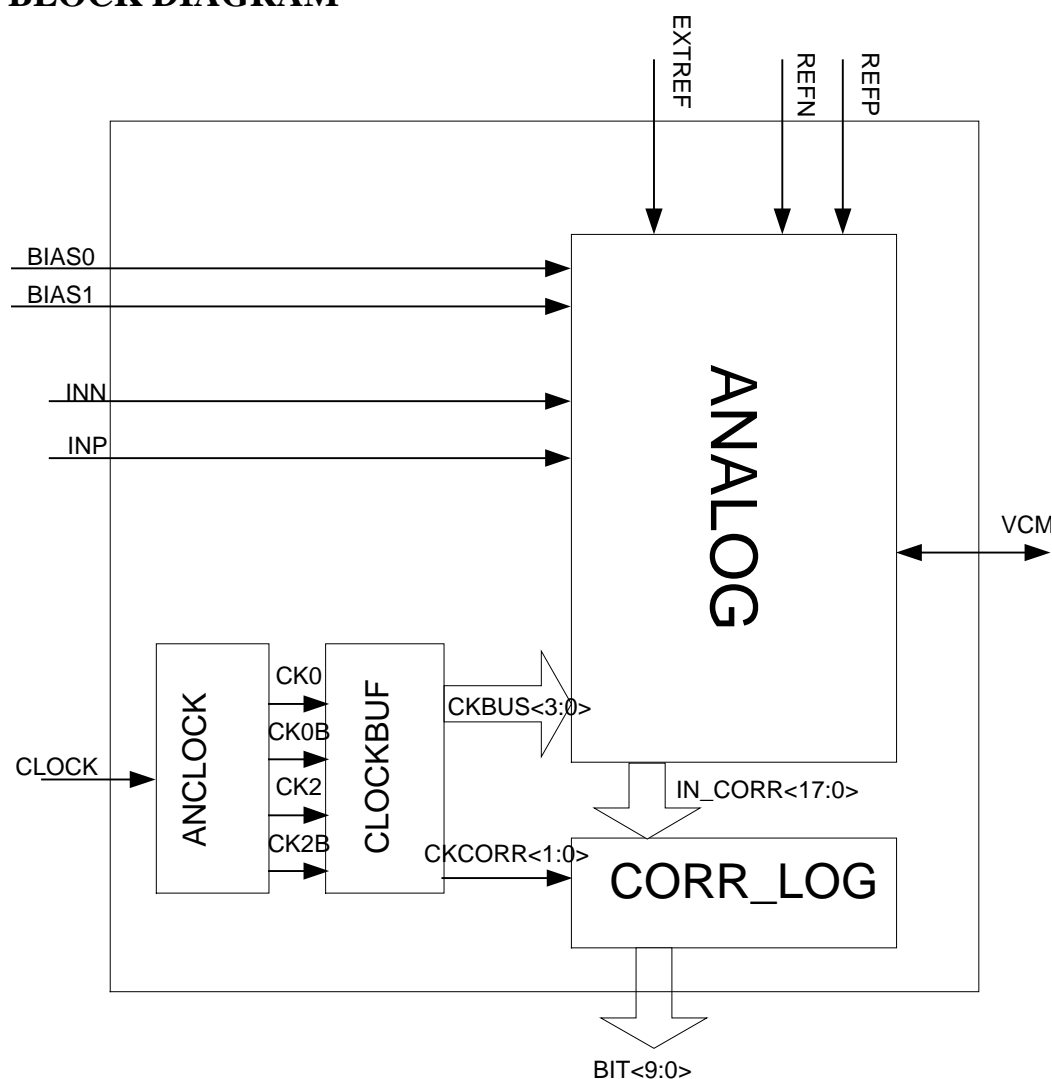
Figure 1. Block diagram nAD1060-18
