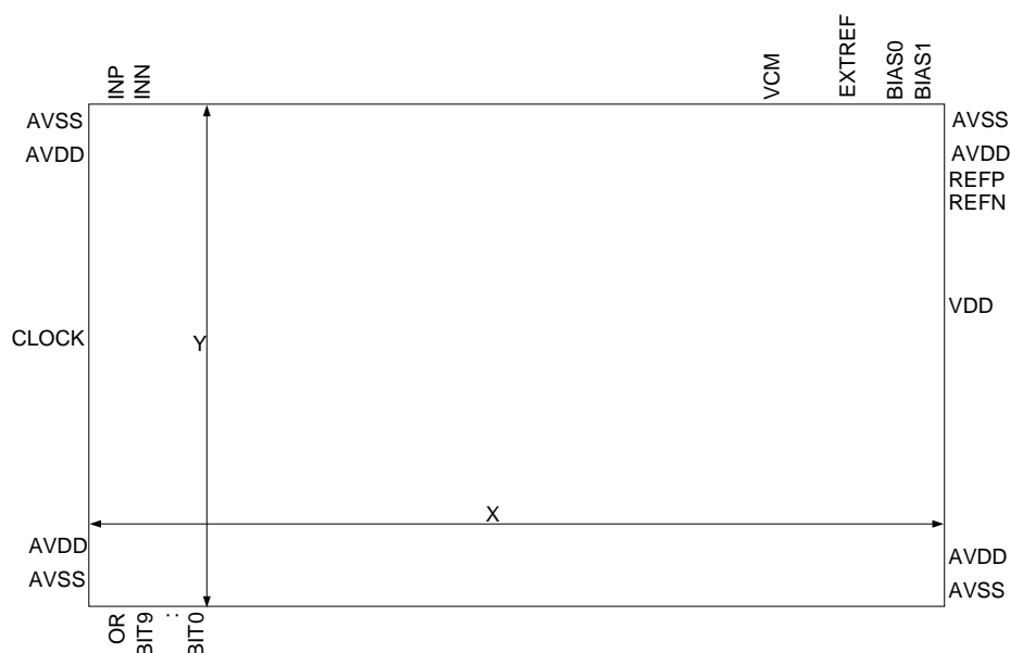
Figure 3. Size and pin placement for nAD1060-18.
