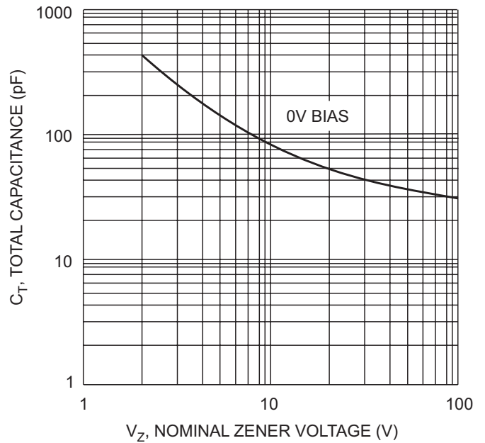
Fig. 2 Typical Capacitance
