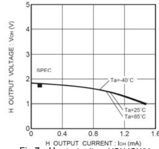
Fig.7 H output voltage V_{OH-IOH}(V_{CC}=1.8V)
