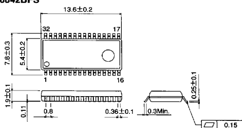
BA6842BFS
