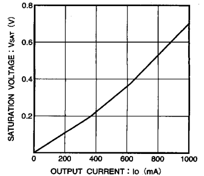
Fig. 3 Low-side output saturation voltage vs. output current
