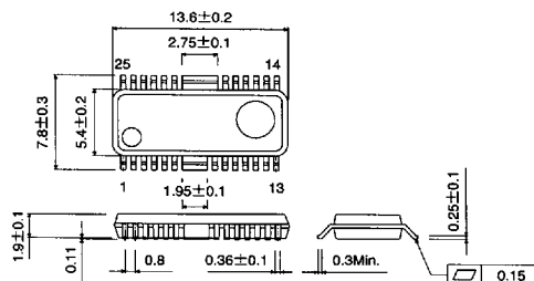
HSOP25
