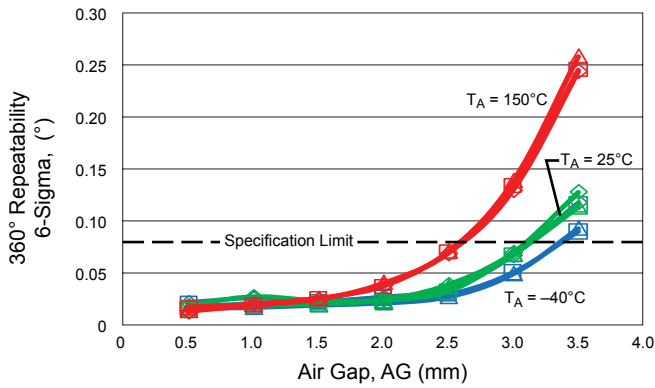
360° Repeatability versus Air Gap Sequential Region, 3 Rising Edges at Each T_A
