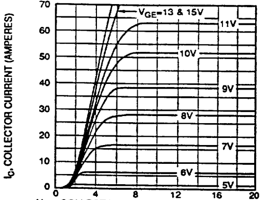
Figure 3, Typical Output Characteristics ( T_J = -55^\circ\text{C} )
