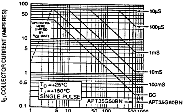
Figure 5, Maximum Forward Bias Safe Operating Area
