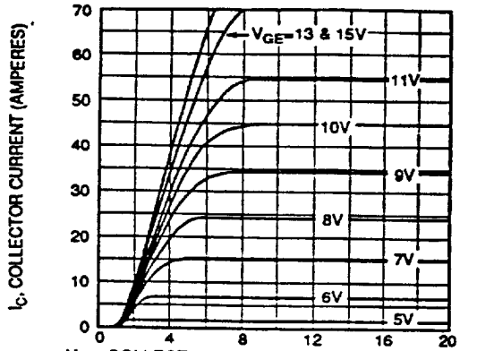
Figure 1, Typical Output Characteristics ( T_J = 25^\circ\text{C} )
