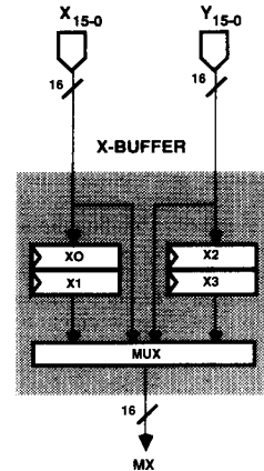
Figure 3. ADSP-1101 X-Buffer
