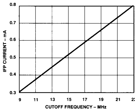
Figure 21. AD896-23 IFP Current vs. Cutoff Frequency
