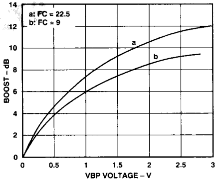
Figure 25. AD896-23 Boost vs. VBP Voltage
