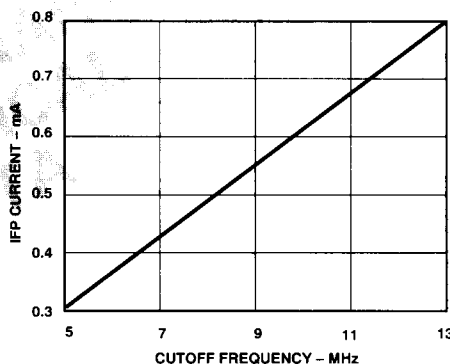
Figure 20. AD896-13 IFP Current vs. Cutoff Frequency
