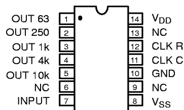
14 Lead PDIP (0.300")
