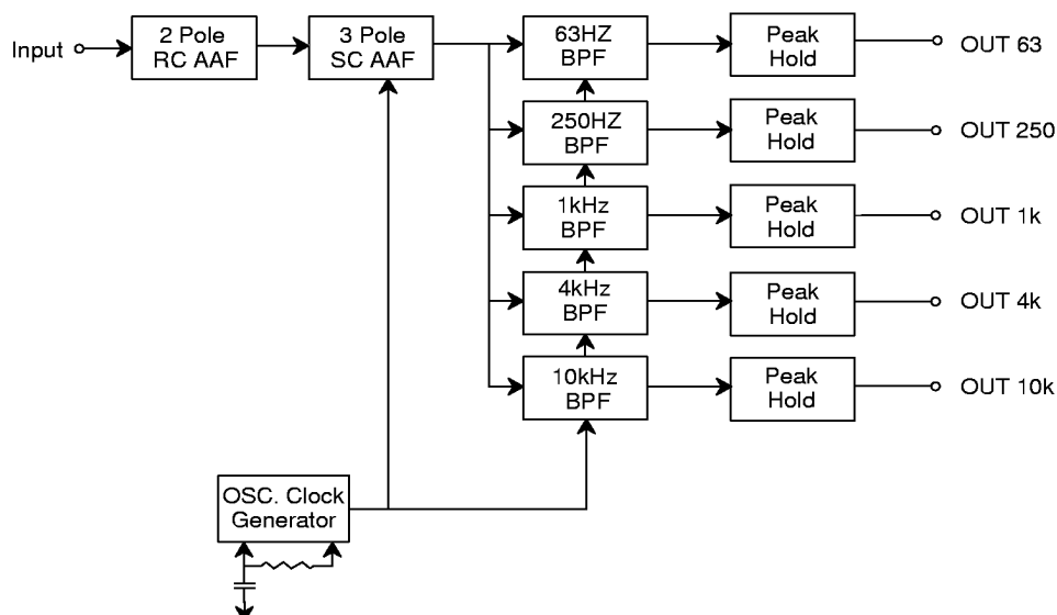
Figure 1. Internal Structure Block Diagram
