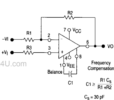
Figure 14. Single-Pole Compensation
