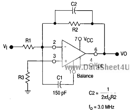
Figure 15. Feedforward Compensation
