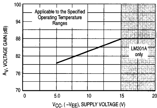
Figure 6. Minimum Voltage Gain
