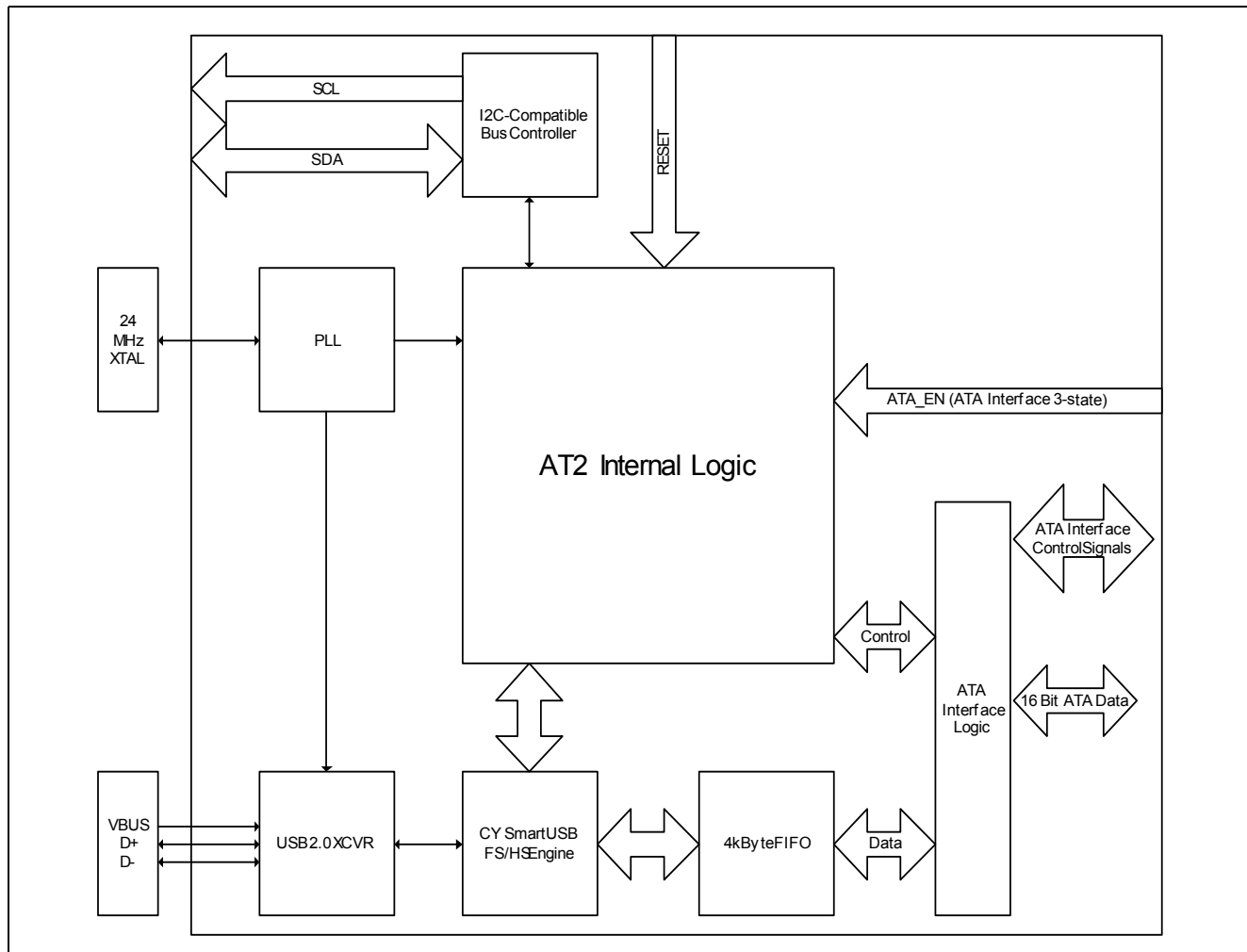
Figure 1-1. Block Diagram
