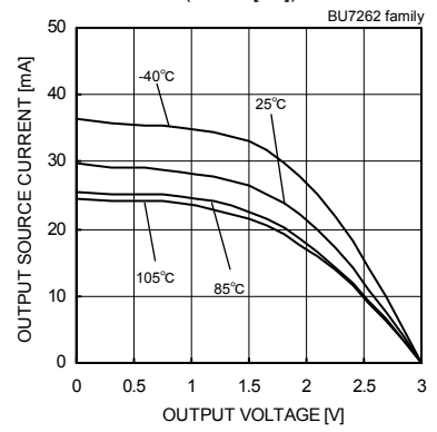
Fig. 32 Output Source Current - Output Voltage (VDD=3.0[V])
