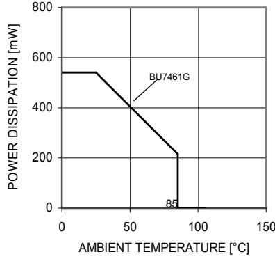
Fig. 93 Derating curve
