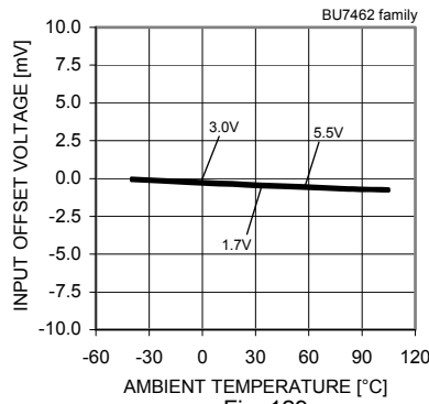
Fig. 129 Input Offset Voltage – Ambient Temperature (Vicm=VDD-1.2[V], VOUT=VDD/2)
