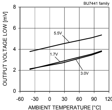
Fig. 146 Output Voltage Low - Ambient Temperature ( R_L=10[k\Omega] )
