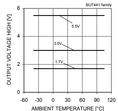
Fig. 144 Output Voltage High - Ambient Temperature ( R_L=10[k\Omega] )
