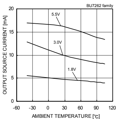
Fig. 33 Output Source Current - Ambient Temperature (VOUT=VDD-0.4[V])
