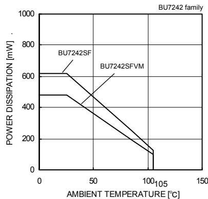
Fig. 71 Derating curve
