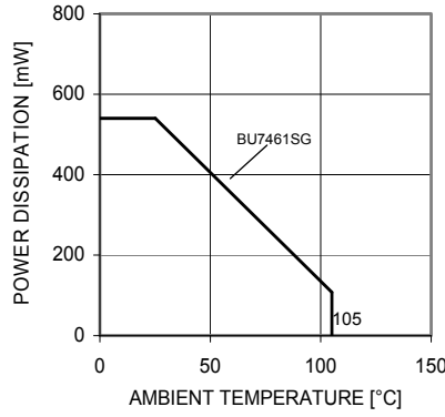
Fig. 94 Derating curve
