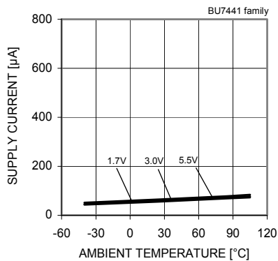
Fig. 142 Supply Current - Ambient Temperature
