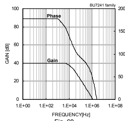
Gain - Frequency
