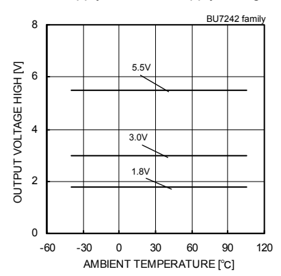
Fig. 75 Output Voltage High - Ambient Temperature (RL=10[kΩ])
