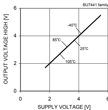
Fig. 143 Output Voltage High - Supply Voltage ( R_L=10[k\Omega] )
