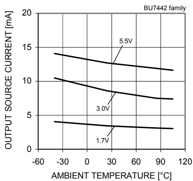
Fig. 171 Output Source Current - Ambient Temperature (VOUT=VDD-0.4[V])
