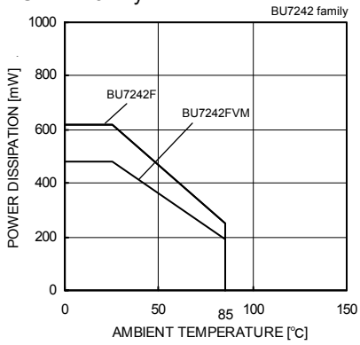
Fig. 70 Derating curve
