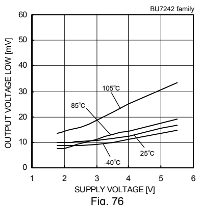
Fig. 76 Output Voltage Low - Supply Voltage (RL=10[kΩ])
