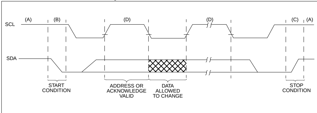
FIGURE 3-2: DATA TRANSFER SEQUENCE ON THE SERIAL BUS
