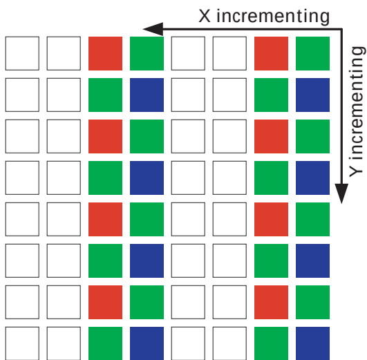
Figure 15: Pixel Readout ( x\_odd\_inc = 3, y\_odd\_inc = 1 )
