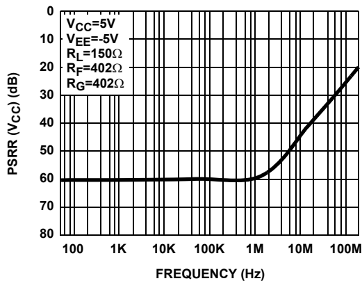
FIGURE 11. PSRR +5V
