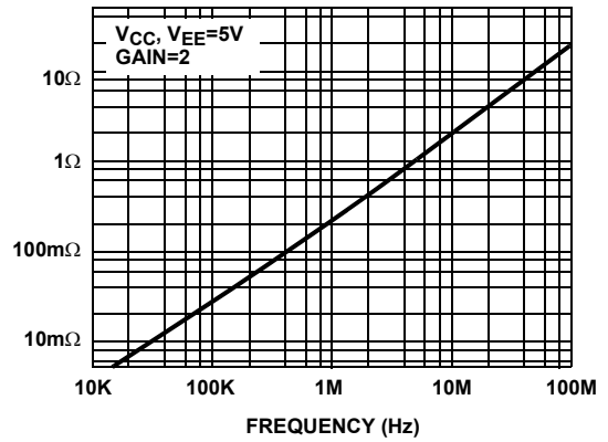
FIGURE 10. CLOSED LOOP OUTPUT IMPEDANCE vs FREQUENCY (6-PIN SOT-23)
