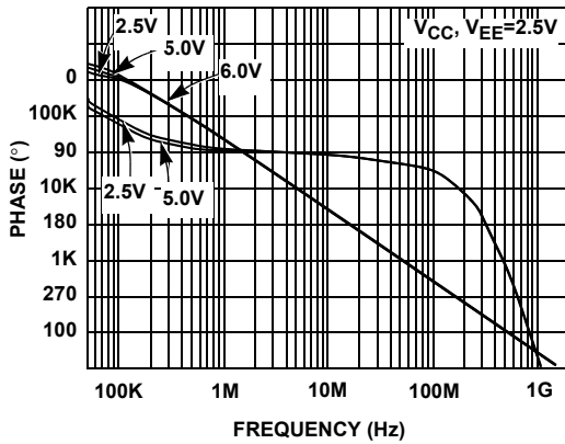
FIGURE 9. TRANSIMPEDANCE MAGNITUDE AND PHASE AS THE FUNCTION OF THE FREQUENCY
