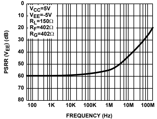
FIGURE 12. PSRR -5V
