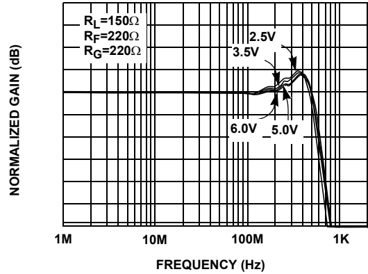
FIGURE 8. INVERTING AMPLIFIER, FREQUENCY RESPONSE AS THE FUNCTION OF V_{CC} , V_{EE} GAIN - 1
