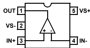
EL5167 (5-PIN SOT-23, SC-70) TOP VIEW
