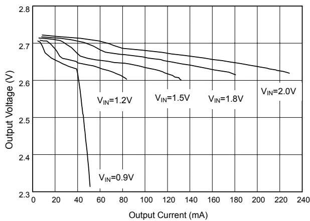
Fig. 6 AIC1642-27 Load Regulation (L=47 \mu H CD54)
