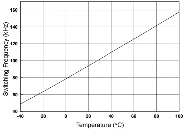
Fig. 22 AIC1642-30 Switching Frequency vs. Temperature
