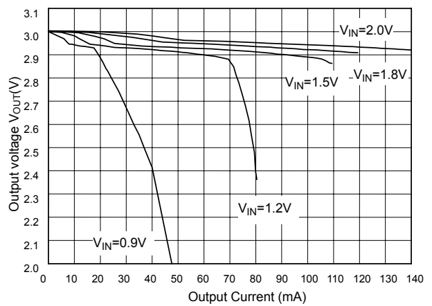
Fig. 15 AIC1642-30 Load Regulation (L=100µH, CD54)
