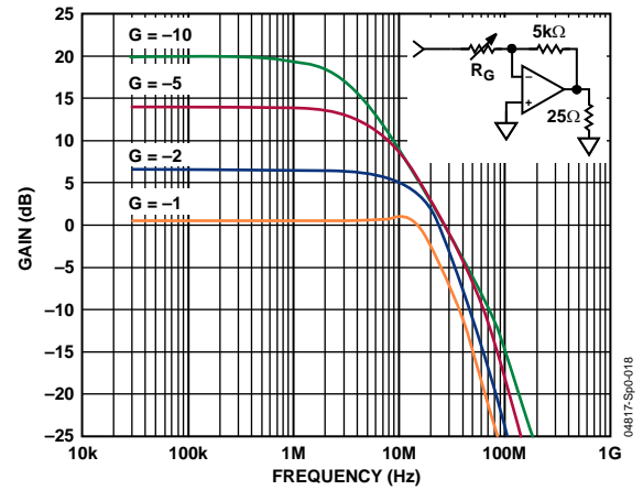
Figure 7. Inverting Large Signal Bandwidth ( V_S = \pm 6V , V_O = 1V p-p, R_L = 25\Omega )
