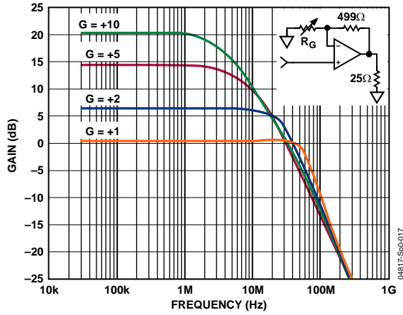
Figure 3. Noninverting Small Signal Bandwidth ( V_S = \pm 6V , V_O = 0.1V p-p, R_L = 25\Omega )
