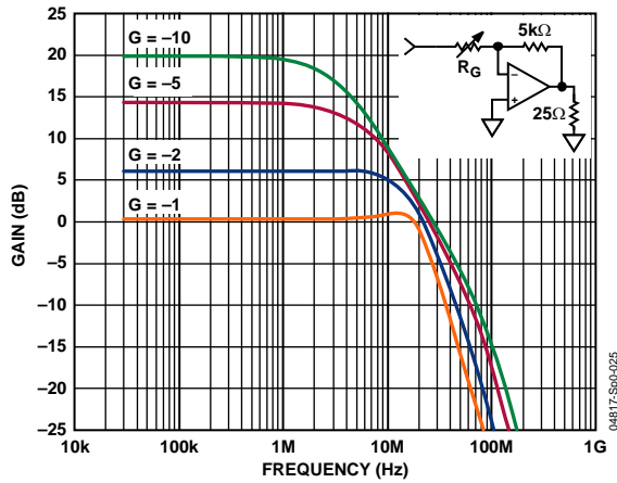
Figure 4. Inverting Small Signal Bandwidth ( V_S = \pm 6V , V_O = 0.1V p-p, R_L = 25\Omega )
