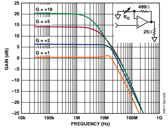
Figure 6. Noninverting Large Signal Bandwidth ( V_S = \pm 6V , V_O = 1V p-p, R_L = 25\Omega )
