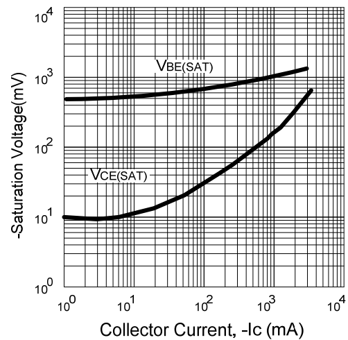
Saturation Voltage
