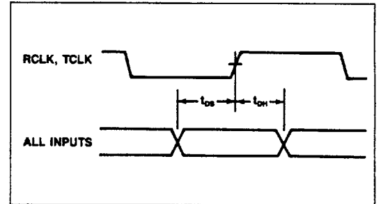
Input Data Setup and Hold Times
