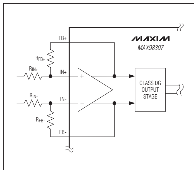
Figure 4. Setting the Voltage Gain of the MAX98307
