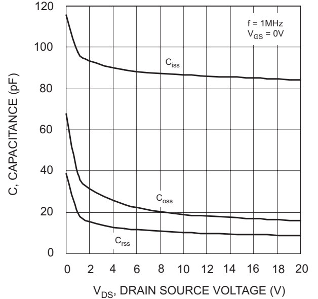
Fig. 12 Capacitance Variation
