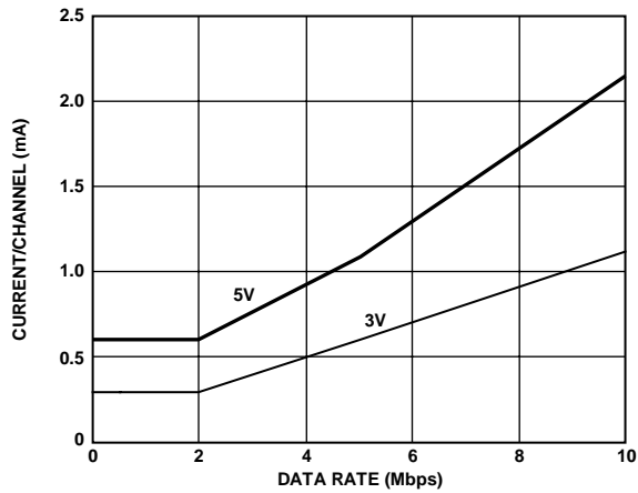
Figure 4. Typical Supply Current per Input Channel vs. Data Rate for 5 V and 3 V Operation
