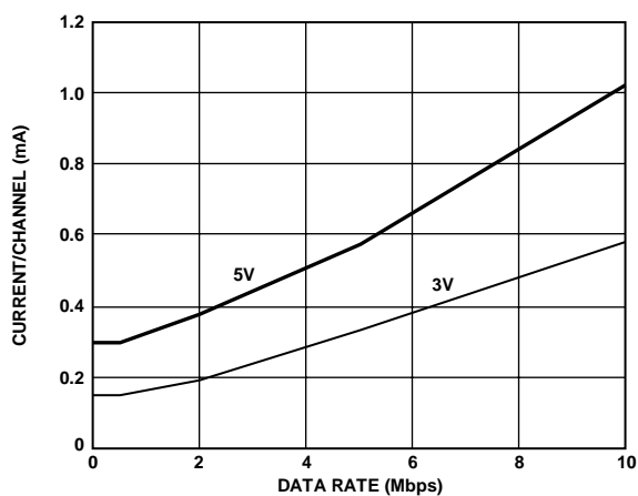
Figure 6. Typical Supply Current per Output Channel vs. Data Rate for 5 V and 3 V Operation (15 pF Output Load)
