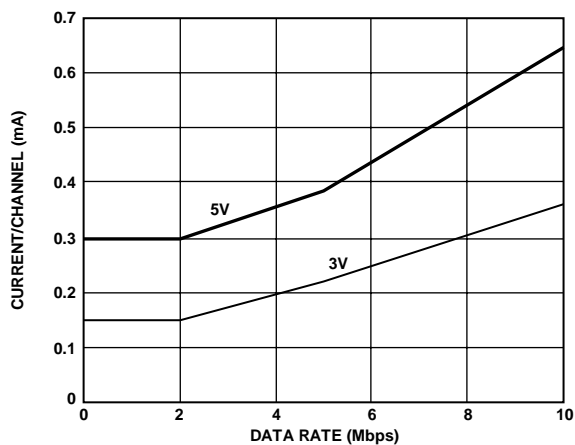
Figure 5. Typical Supply Current per Output Channel vs. Data Rate for 5 V and 3 V Operation (No Output Load)
