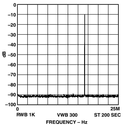
TPC 18. f_{MCLK} = 50 \text{ MHz} ; f_{OUT} = 16.667 \text{ MHz} = f_{MCLK}/3 , Frequency Word = 5555555
