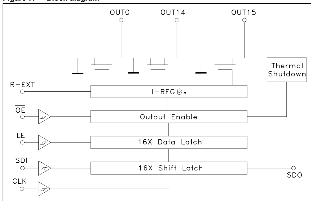
Figure 7. Block diagram
