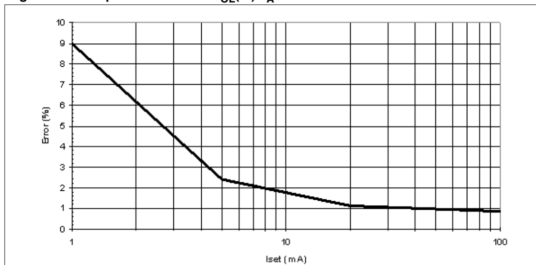
Figure 13. Output current vs \pm \Delta I_{OL}(\%) T_A = 25^\circ\text{C}
