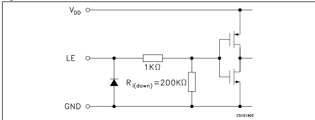
Figure 4. LE terminal
