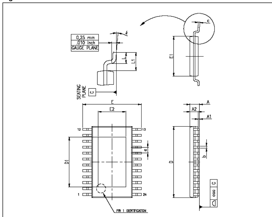
Figure 26. TSSOP24 dimensions
