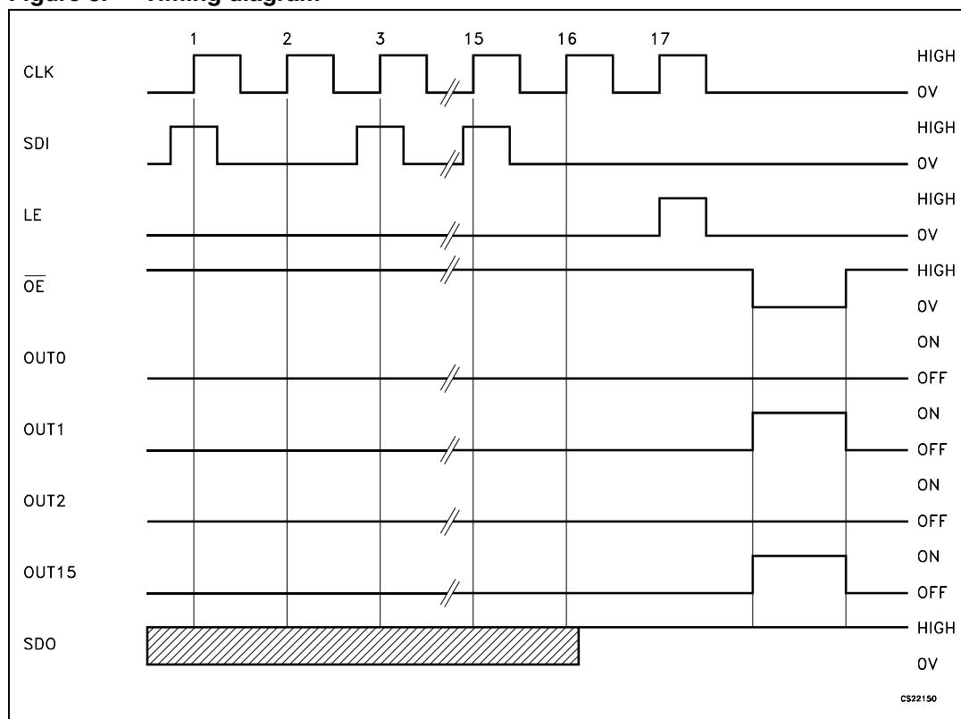
Figure 8. Timing diagram
