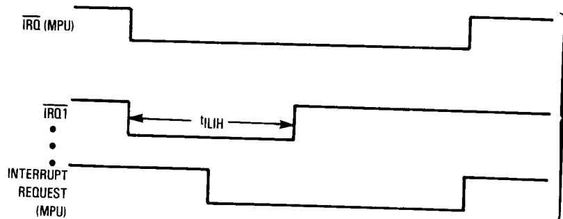
Figure 14. External Interrupt
