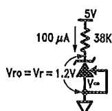
FIGURE 3. 1.2V Reference
