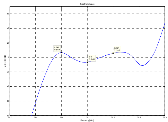
Phase Linearity(f0±0.1MHz)
