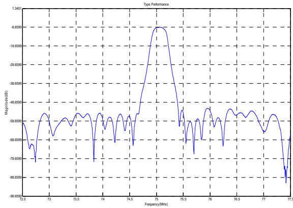
Frequency Respond
