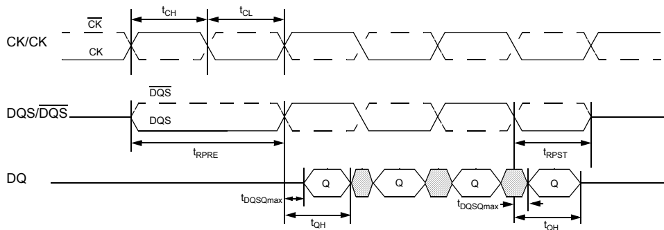
Figure 4 - Data Output (Read) Timing
