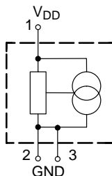
Fig. 1-4: Pin configuration
