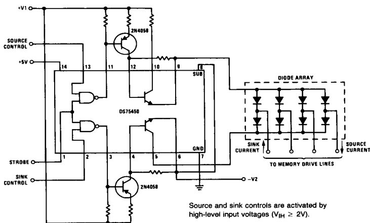
FIGURE 24. Core Memory Driver
