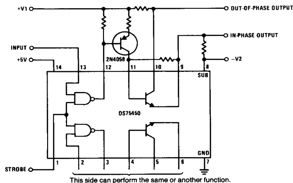
FIGURE 22. Floating Switch
