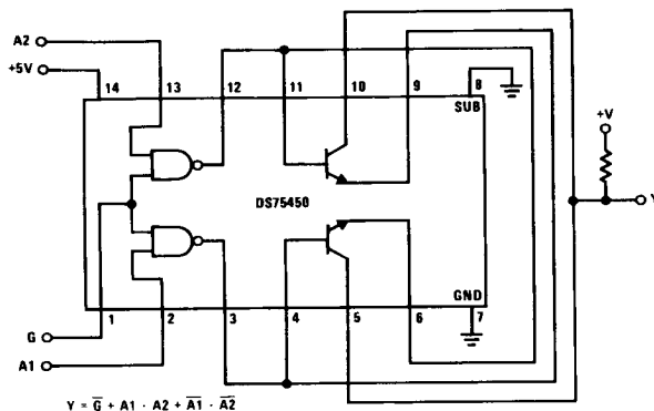
FIGURE 20. Gated Comparator
