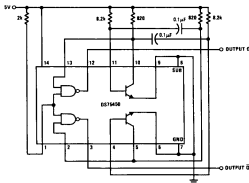
FIGURE 23. Square-Wave Generator
