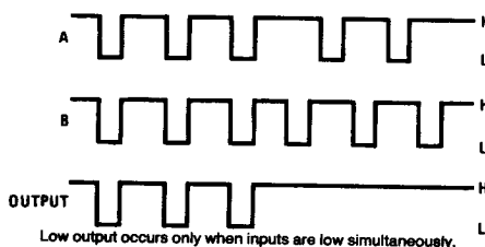
FIGURE 33. In-Phase Detector
