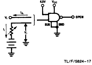
FIGURE 3. V_I , I_{IL}
