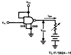
FIGURE 2. V_{IL} , V_{OH}
