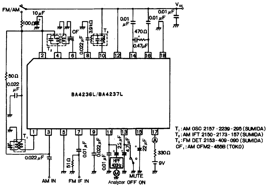
Figure 1 Test circuit
