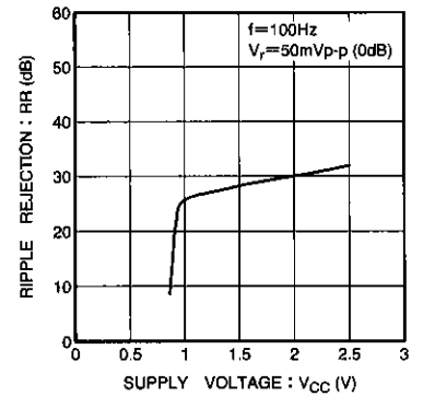
Fig. 22 Ripple rejection ratio vs. supply voltage
